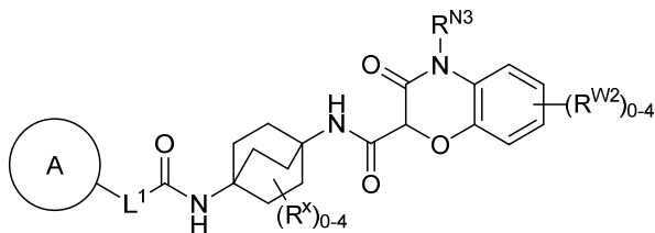
Formula (I-c-4)
