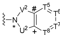
Formula (W-b)
