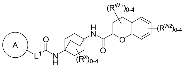
Formula (I-c-3)
