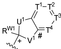
Formula (W-a)
