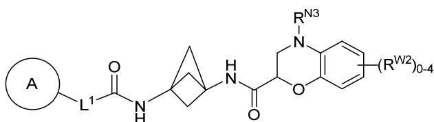
Formula (I-d-2)
