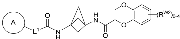
Formula (I-d-5)
