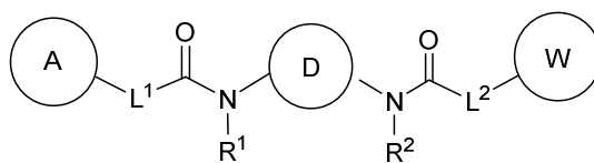
Formula (I-a)
