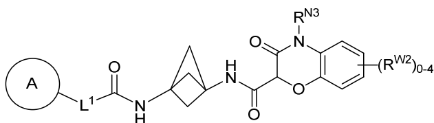
Formula (I-d-4)
