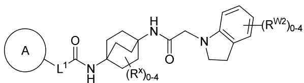
Formula (I-c-9)
