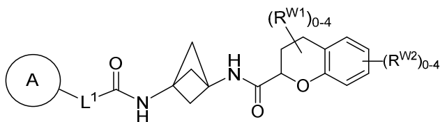
Formula (I-d-3)
