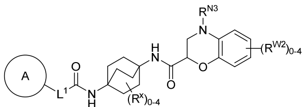
Formula (I-c-2)
