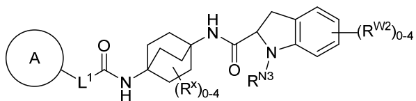
Formula (I-c-6)
