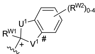
Formula (W-a-1).
