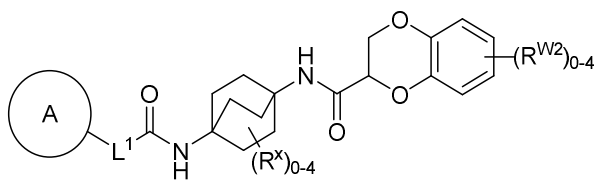
Formula (I-c-5)
