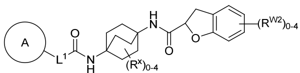
Formula (I-c-7)
