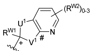
Formula (W-a-5).
