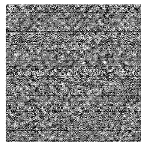
Correlated patterns
