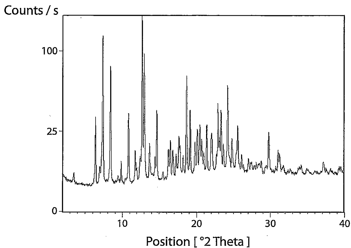
Fig. 1A (MONOSACCHARIN SALT)
