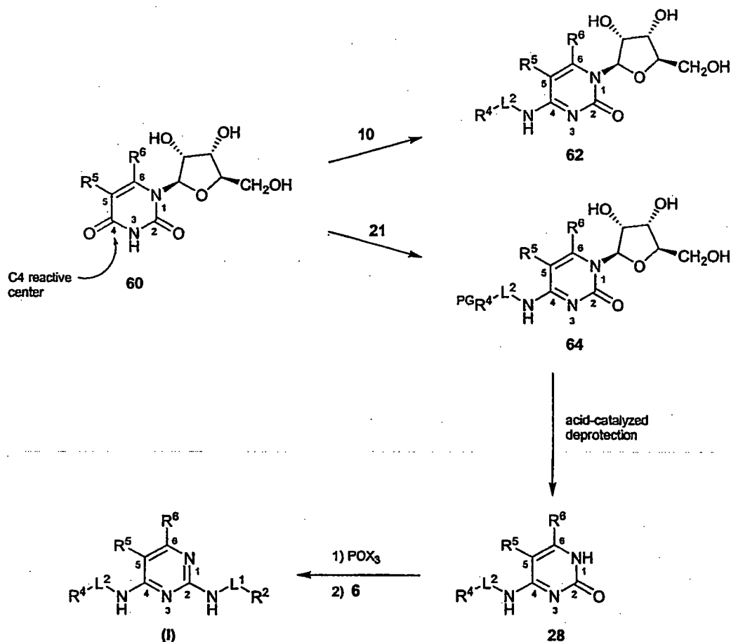
Scheme (VI)
