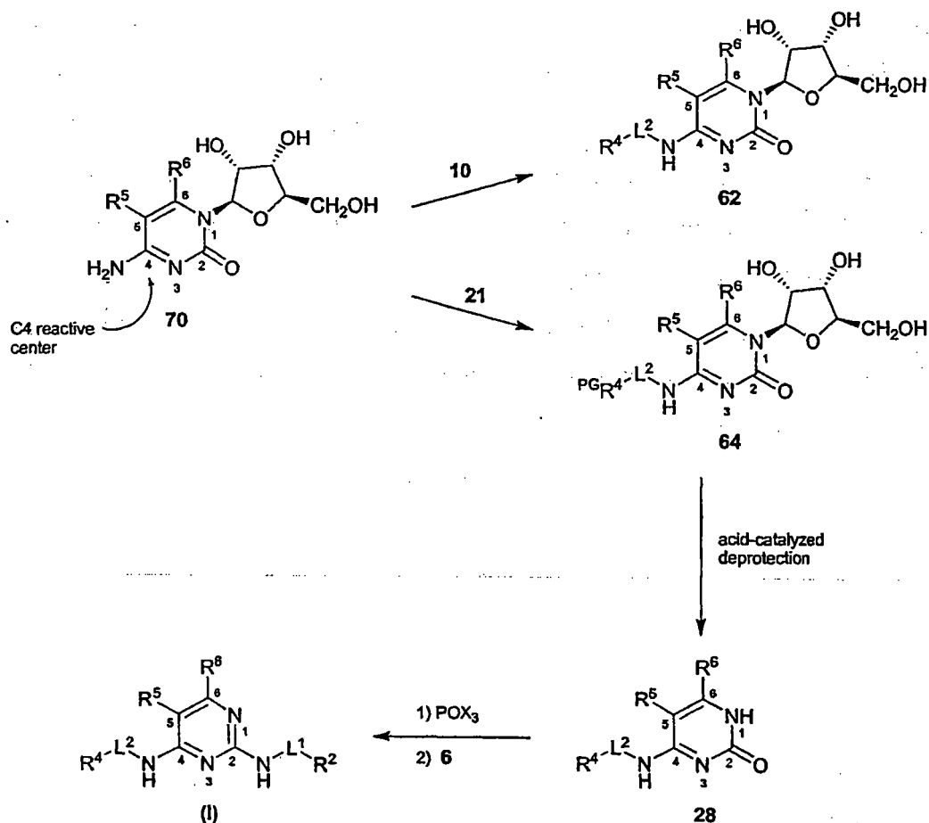
Scheme (VII)
