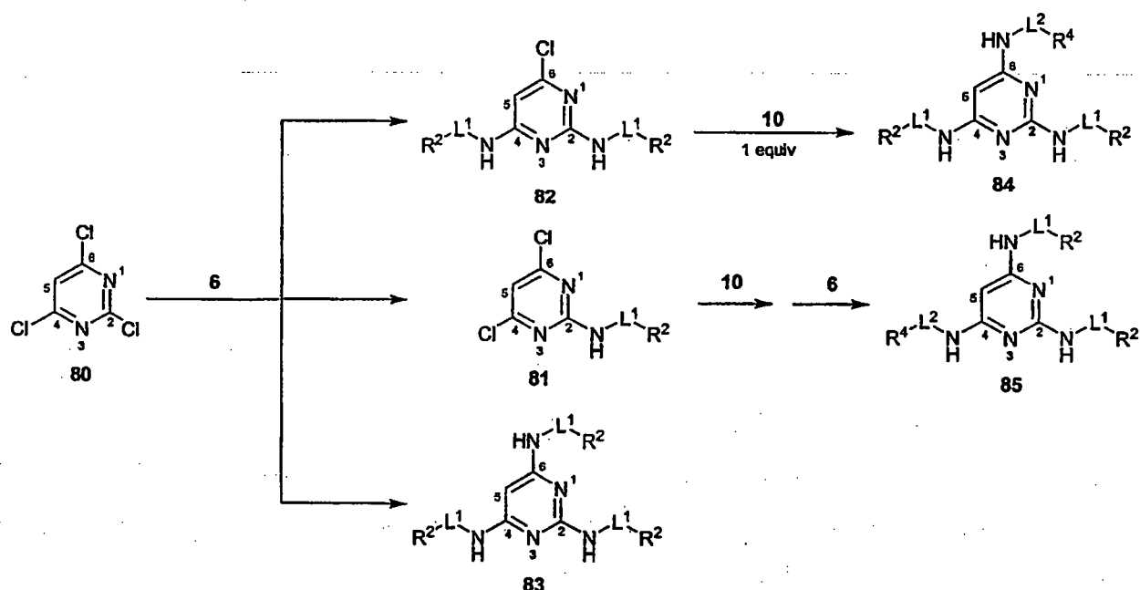
Scheme (VIII)
