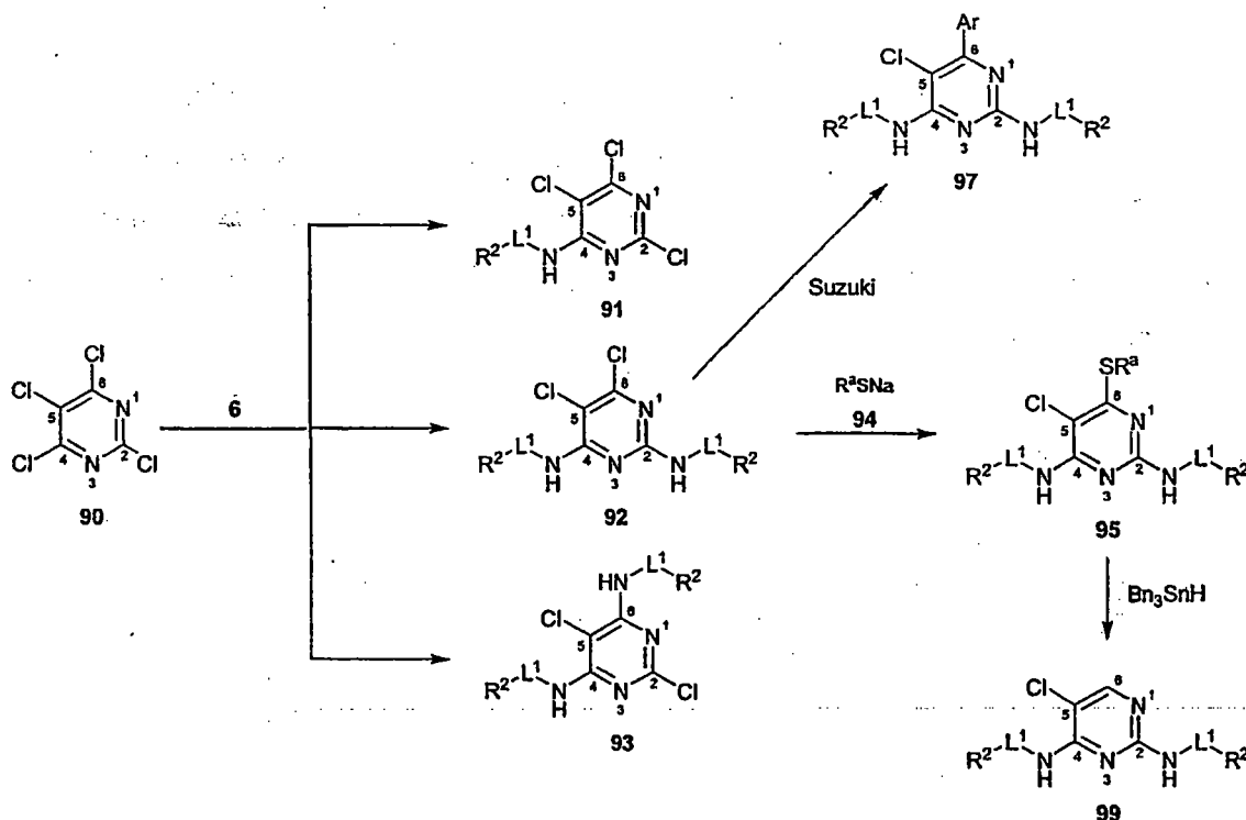
Scheme (IX)
