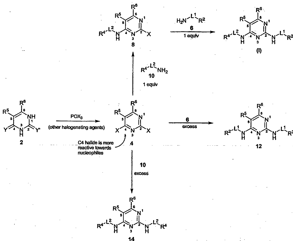
Scheme (I)
