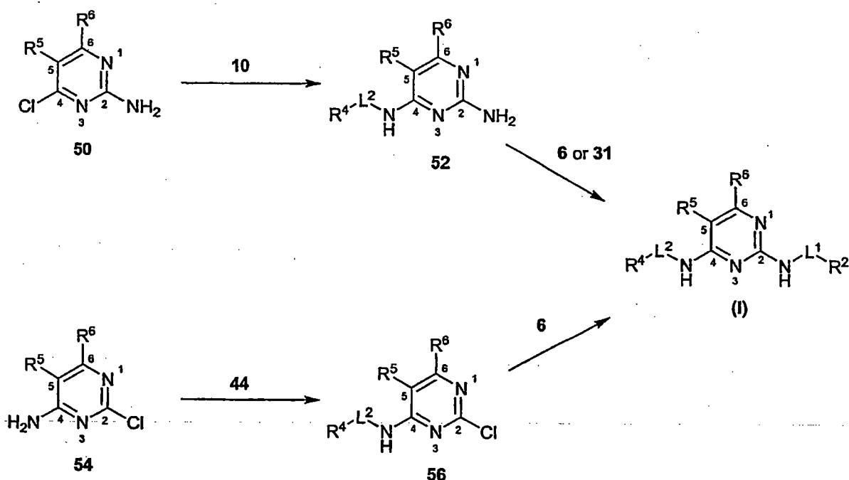
Scheme (V)
