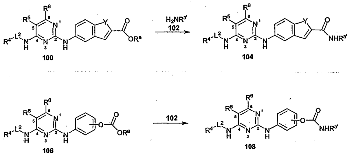
Scheme (X)
