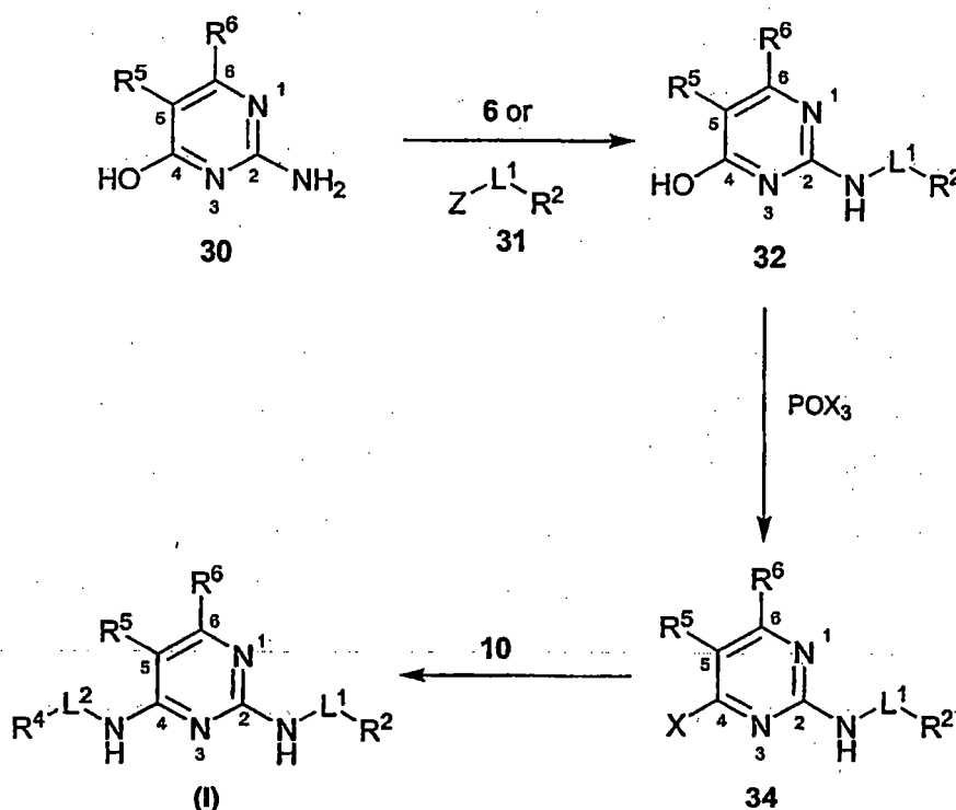
Scheme (III)
