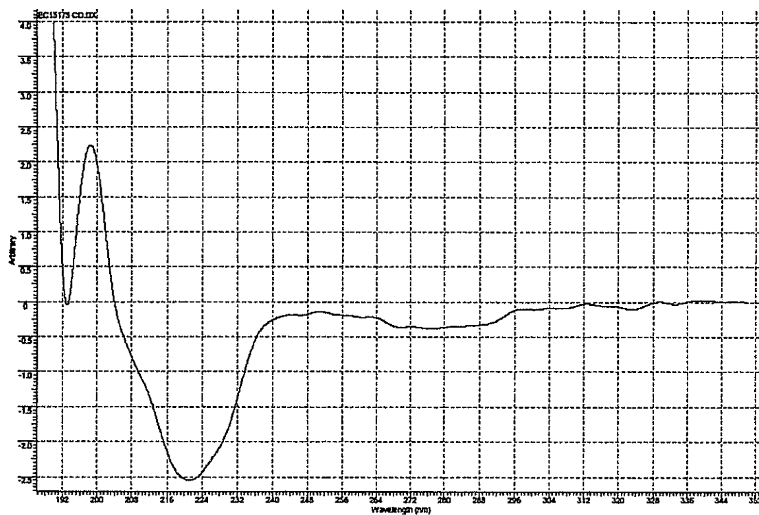
Figure 1: CD spectrum of ( R )-4-(4-bromophenyl)-2,2-dimethyl-1,3-dioxolane
