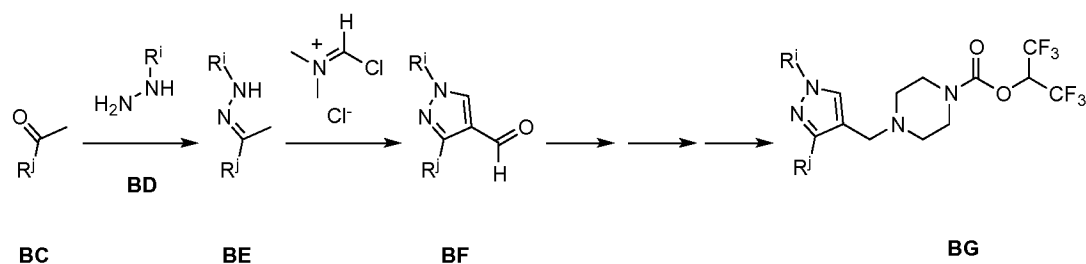
SCHEME 14
