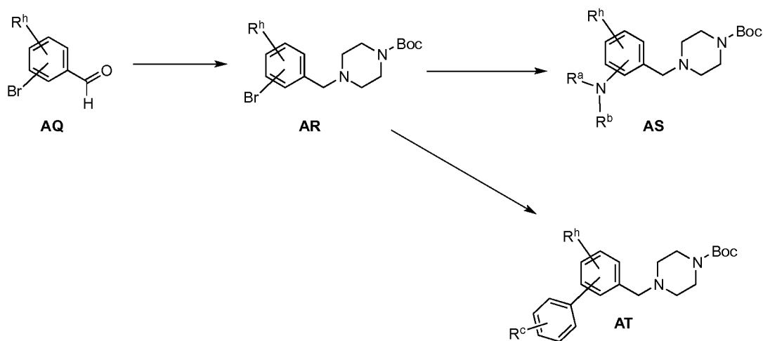
SCHEME 11
