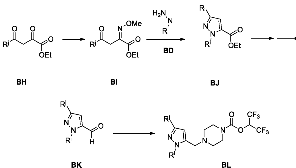
SCHEME 15
