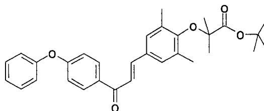
1-(4-Phenyloxyphenyl)-3-(4-carboxydimethylmethoxy-3,5-dimethylphenyl)prop-2-en-1-one :
