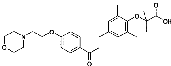
1-(4-(Morpholin-4-ylethyloxy)phenyl)-3-(4-carboxydimethylmethoxy-3,5-dimethylphenyl)prop-2-en-1-one :
