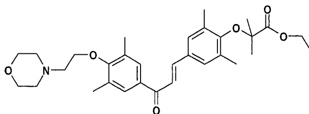
10 1-(3,5-Dimethyl-4-(morpholin-4-ylethyloxy)phenyl)-3-(4-carboxydimethylmethoxy-3,5-dimethylphenyl)prop-2-en-1-one :
