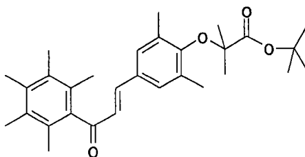
1-(2,3,4,5,6-Pentamethylphenyl)-3-(4-carboxydimethylmethoxy-3,5-dimethylphenyl)prop-2-en-1-one :
