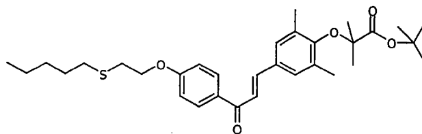
1-(4-(Pentylthioethyloxy)phenyl)-3-(4-carboxydimethylmethoxy-3,5-dimethylphenyl)prop-2-en-1-one :
