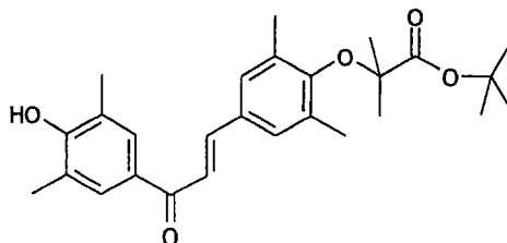
1-(4-Hydroxy-3,5-dimethylphenyl)-3-(4-carboxydimethylmethoxy-3,5-dimethylphenyl)prop-2-ene-1-one :
