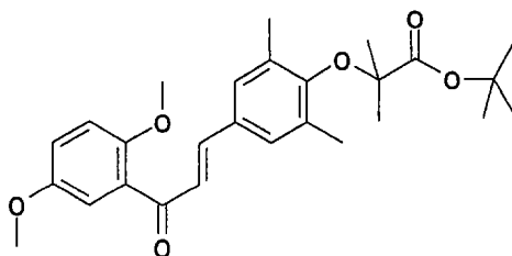
1-(2,5-Dimethoxyphenyl)-3-(4-carboxydimethylmethoxy-3,5-dimethylphenyl)prop-2-en-1-one :
