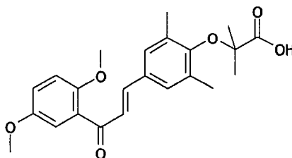
5 1-(3,5-Dimethyl-4-(morpholin-4-ylethyloxy)phenyl)-3-(4-ethyloxycarbonyldimethylmethoxy-3,5-dimethylphenyl)prop-2-en-1-one hydrochloride :
