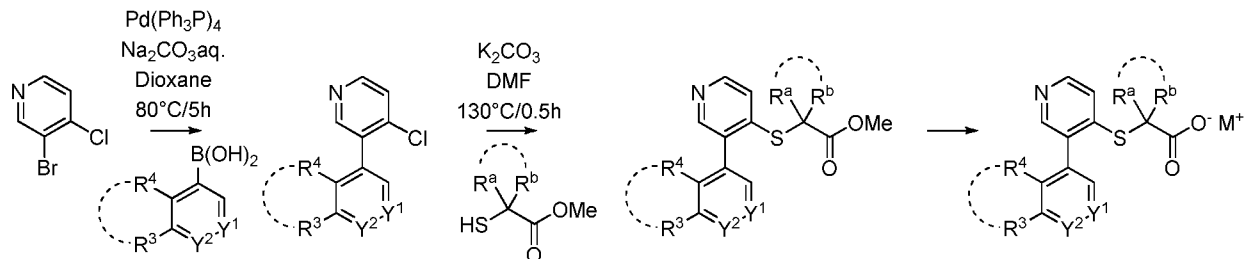
Scheme I-B-b:
