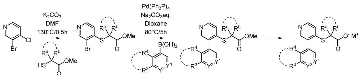
Scheme I-B-c:
