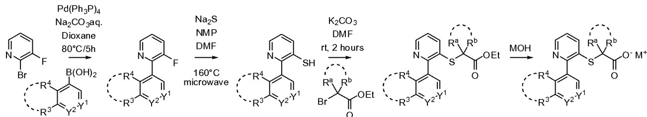
Scheme I-A-b:
