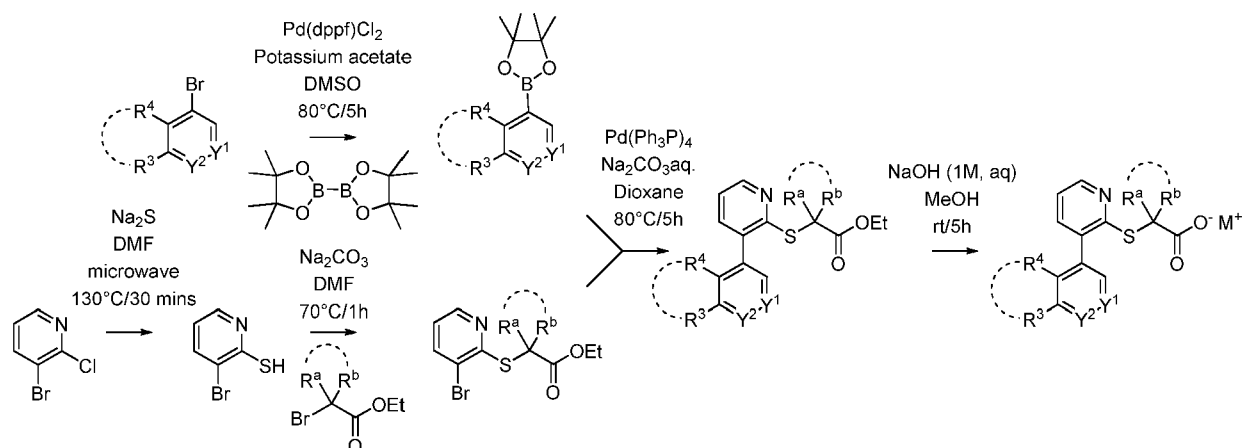
Scheme I-D-a:
