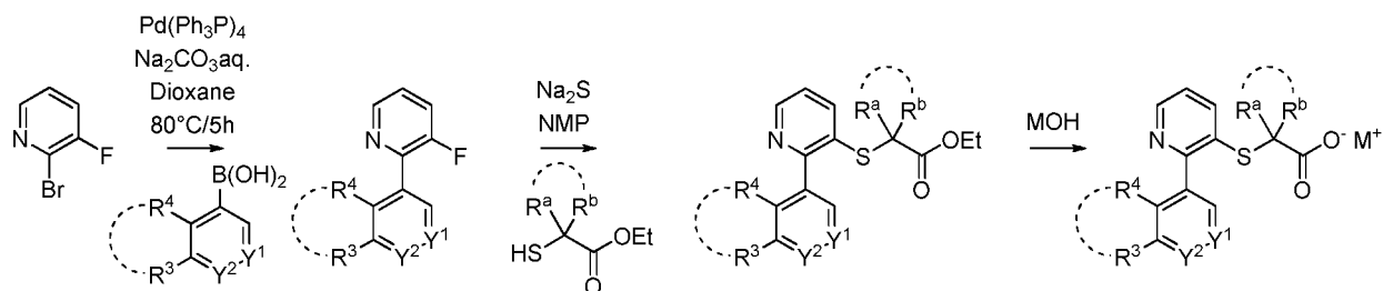
Scheme I-A-b:
