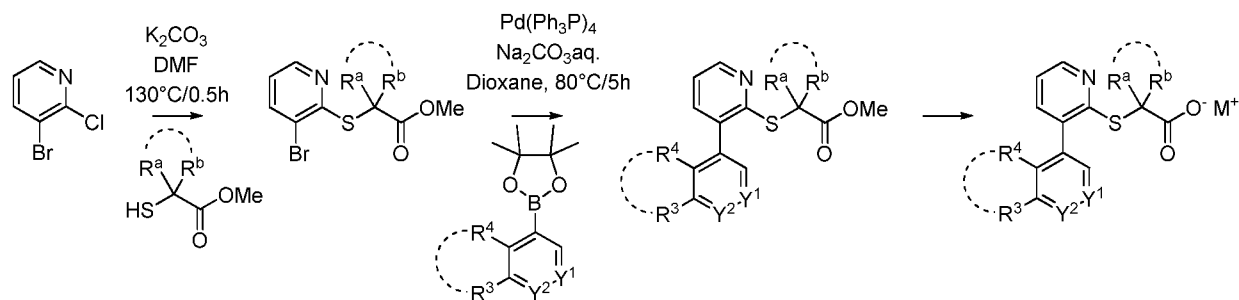
Scheme I-D-c:
