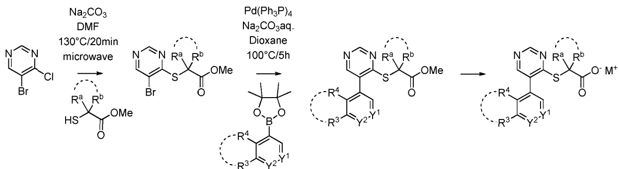
Scheme I-F-a:
