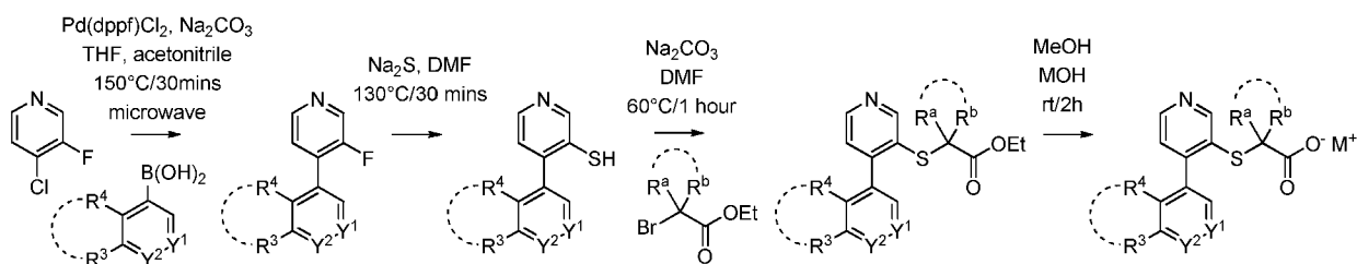
Scheme I-C:
