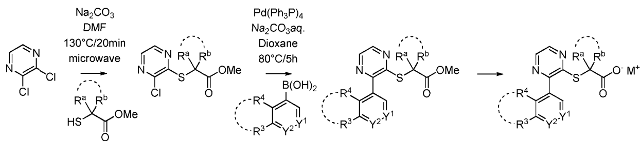
Scheme I-F-a:
