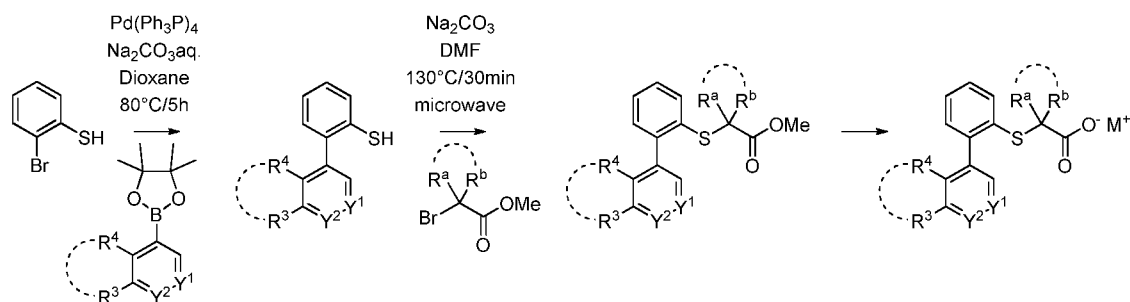
Scheme I-H-a:
