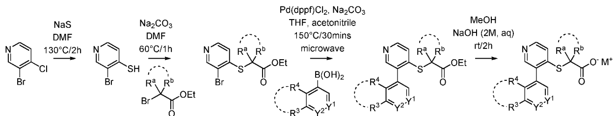
Scheme I-B-b:
