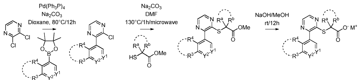
Scheme I-E-a:
