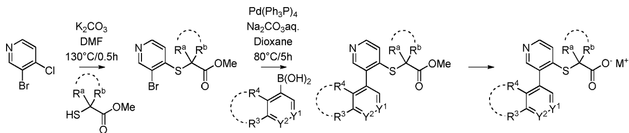
10 Scheme I-B-c:
