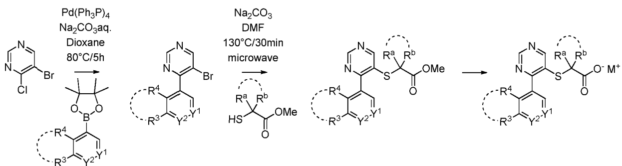
Scheme I-G-a:
