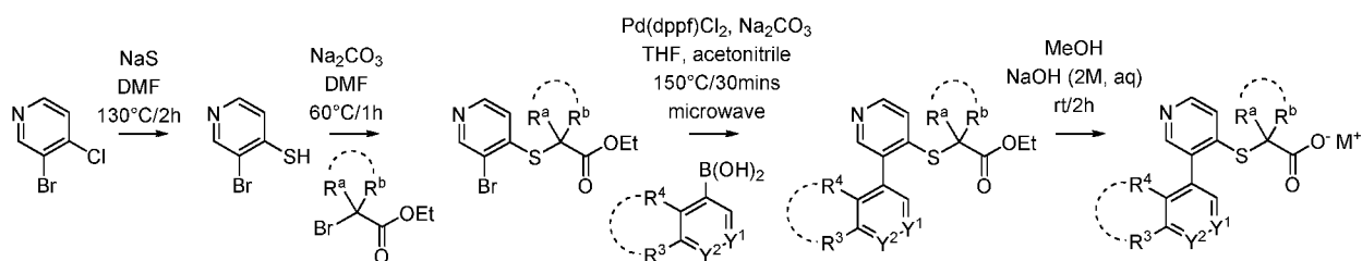
Scheme I-B-a:
