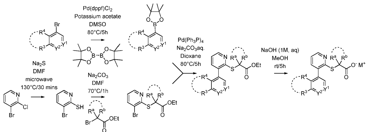
Scheme I-D-b:
