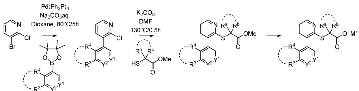
Scheme I-D-c:
