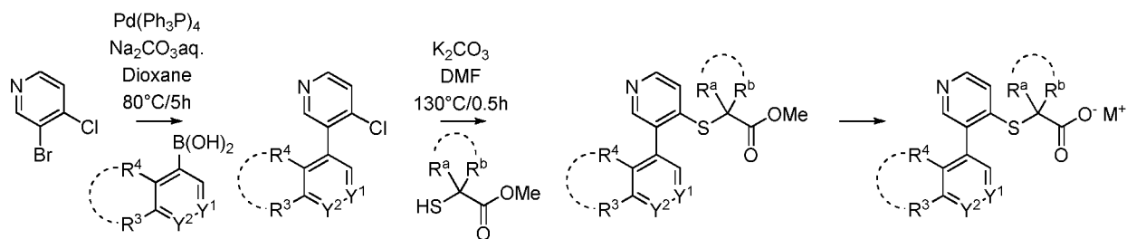
Scheme I-B-b:
