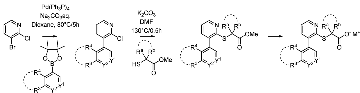
Scheme I-D-c:
