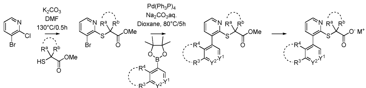
Scheme I-E-a:
