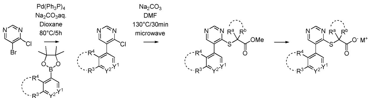
Scheme I-F-b:
