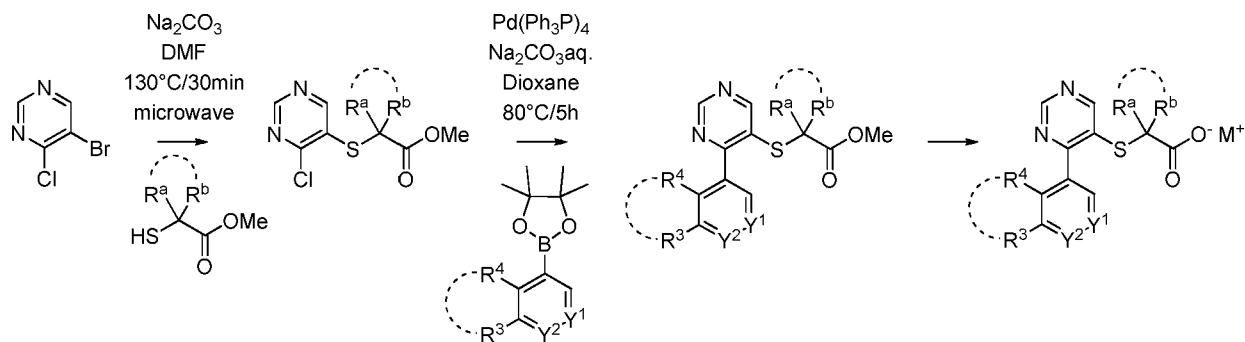
Scheme I-H-a:
