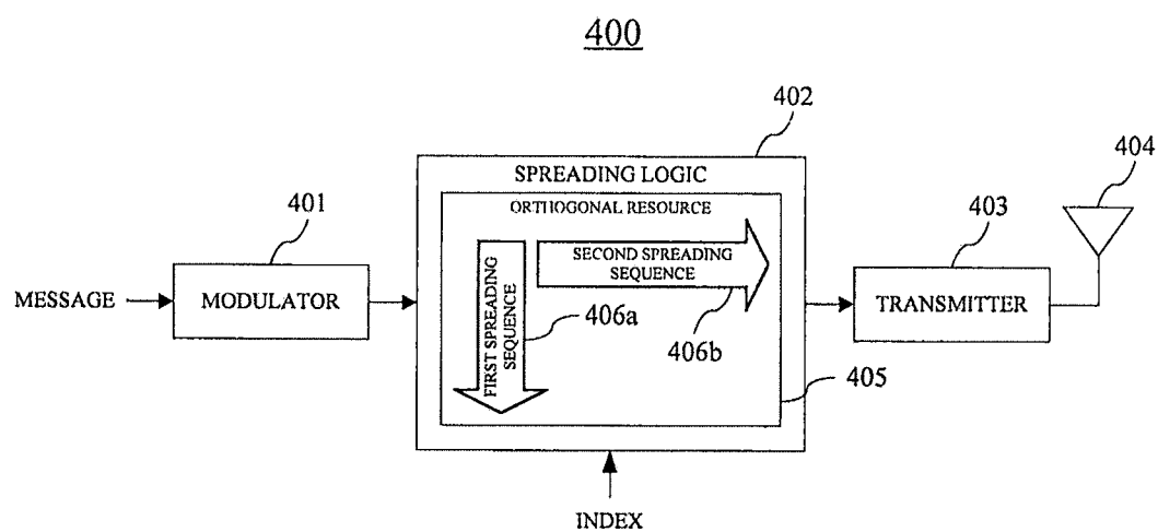
FIG. 4 (PRIOR ART)
