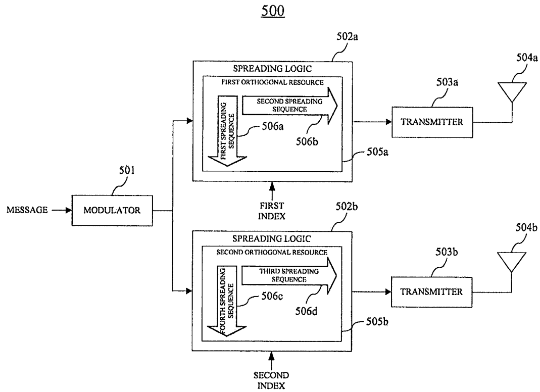
FIG. 5 (PRIOR ART)
