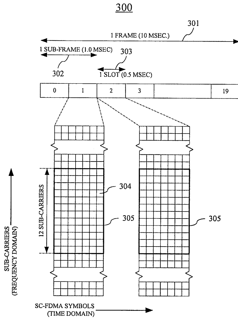
FIG. 3 (PRIOR ART)
