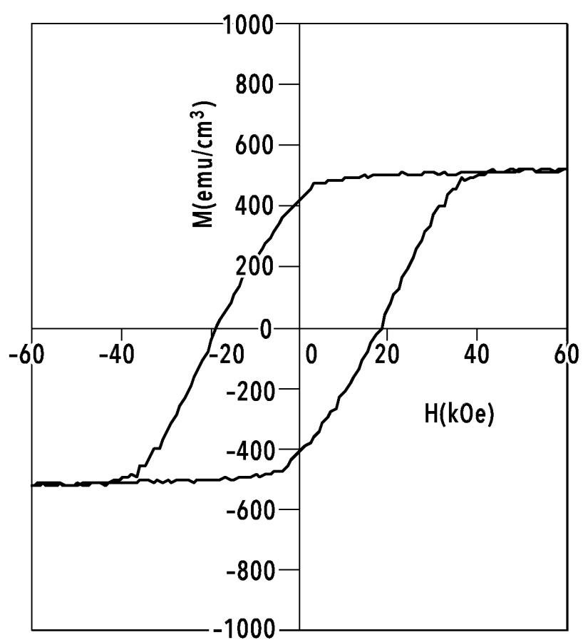
MAGNETIZATION CURVE OF SAMPLE No. = 1-3 IN EXAMPLE 1
