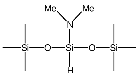
3-dimethylamino-1,1,1,5,5,5- hexamethyltrisiloxane
