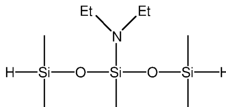
3-diethylamino-1,1,3,5,5-pentamethyltrisiloxane
