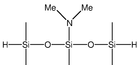
3-dimethylamino-1,1,3,5,5-pentamethyltrisiloxane
