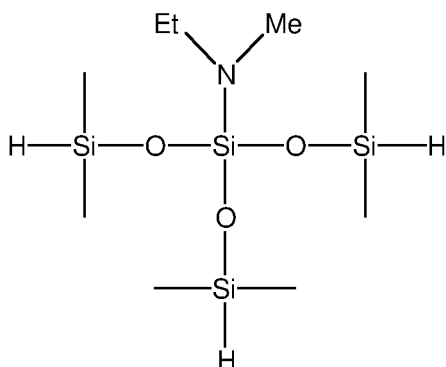
3-ethylmethylamino-3-(dimethylsiloxy)-1,1,5,5-tetramethyltrisiloxane
