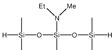
3-ethylmethylamino-1,1,3,5,5-pentamethyltrisiloxane
