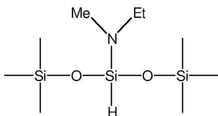
3-ethylmethylamino-1,1,1,5,5,5- hexamethyltrisiloxane
