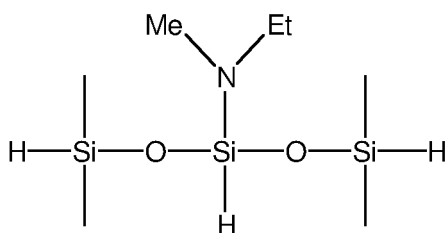
3-ethylmethylamino-1,1,5,5-tetraamethyltrisiloxane
