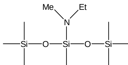
Structure I
