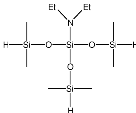
3-diethylamino-3-(dimethylsiloxy)-1,1,5,5-tetramethyltrisiloxane
