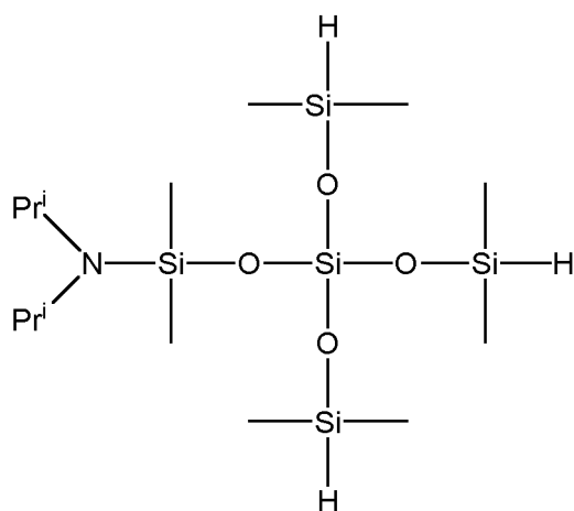
1-di-iso-propylamino-3,3-bis(dimethylsiloxy)-1,1,5,5-tetramethyltrisiloxane
