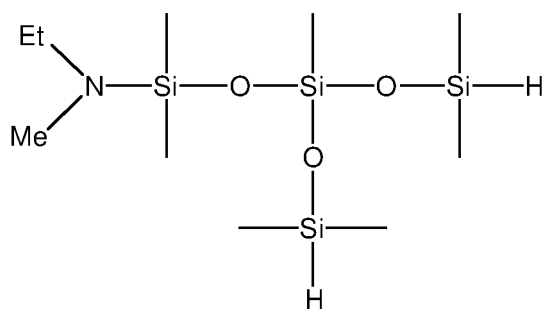
1-ethylmethylamino-3-(dimethylsiloxy)- 1,1,3,5,5-pentamethyltrisiloxane
