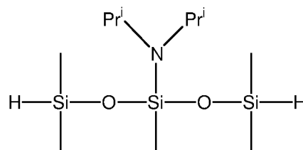
3-di-iso-propylamino-1,1,3,5,5-pentamethyltrisiloxane
