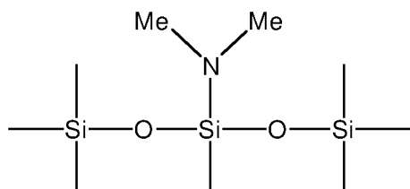
3-dimethylamino-1,1,1,3,5,5,5-heptamethyltrisiloxane
