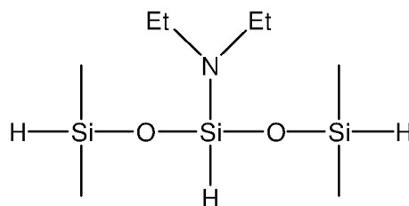
3-diethylamino-1,1,5,5,5-tetramethyltrisiloxane
