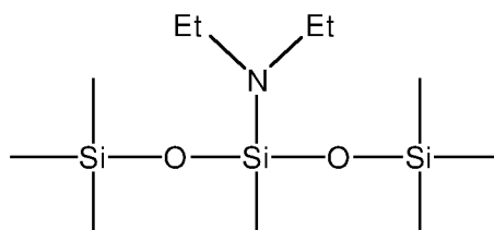
3-diethylamino-1,1,1,3,5,5,5-heptamethyltrisiloxane
