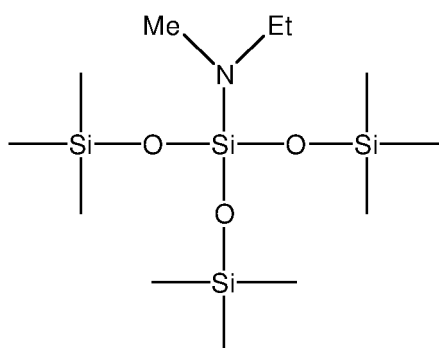
3-ethylmethylamino-3-(trimethylsiloxy)- 1,1,1,5,5,5-hexamethyltrisiloxane
