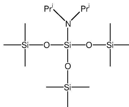
3-di-iso-propylamino-3-(trimethylsiloxy)- 1,1,1,5,5,5-hexamethyltrisiloxane
