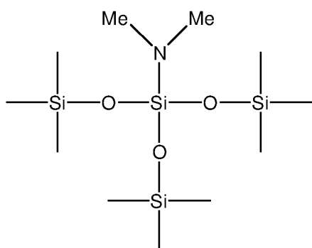
3-dimethylamino-3-(trimethylsiloxy)- 1,1,1,5,5,5-hexamethyltrisiloxane
