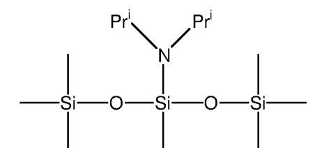
3-di-iso-propylamino-1,1,1,3,5,5,5-heptamethyltrisiloxane
