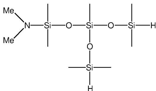
1-dimethylamino-3-(dimethylsiloxy)-1,1,3,5,5-pentamethyltrisiloxane
