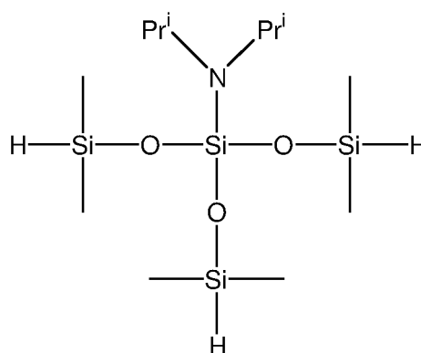
3-di-iso-propylamino-3-(dimethylsiloxy)-1,1,5,5-tetramethyltrisiloxane
