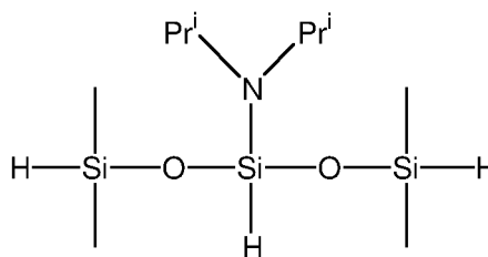
3-di-iso-propylamino-1,1,5,5-tetramethyltrisiloxane
