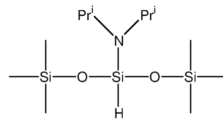
3-di-iso-propylamino-1,1,1,3,5,5,5- hexamethyltrisiloxane
