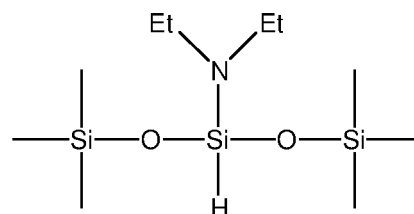
3-diethylamino-1,1,1,5,5,5- hexamethyltrisiloxane
