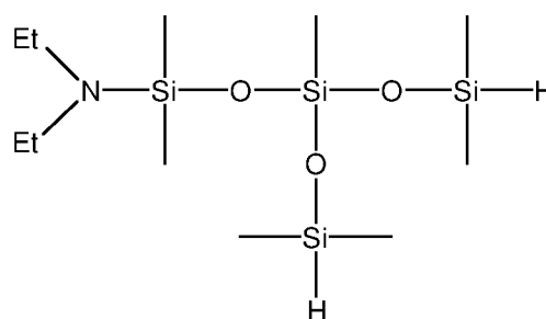
1-diethylamino-3-(dimethylsiloxy)-1,1,3,5,5-pentamethyltrisiloxane
