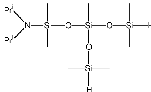
1-di-iso-propylamino-3-(dimethylsiloxy)- 1,1,3,5,5-pentamethyltrisiloxane
