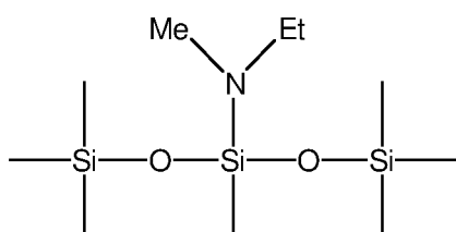
3-ethylmethylamino-1,1,1,3,5,5,5-heptamethyltrisiloxane
