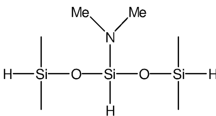
3-dimethylamino-1,1,5,5,5- tetramethyltrisiloxane
