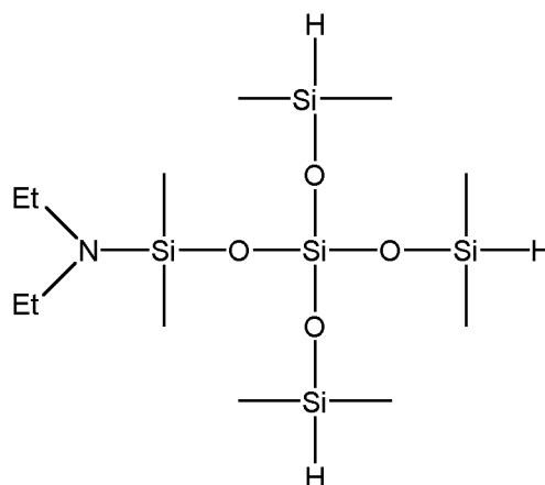
1-diethylamino-3,3-bis(dimethylsiloxy)-1,1,5,5-tetramethyltrisiloxane
