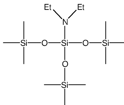
3-diethylamino-3-(trimethylsiloxy)-1,1,1,5,5,5- hexamethyltrisiloxane
