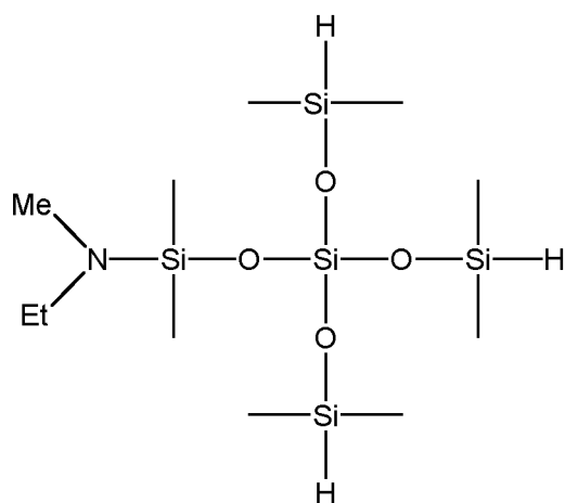
1-ethylmethylamino-3,3-bis(dimethylsiloxy)-1,1,5,5-tetramethyltrisiloxane
