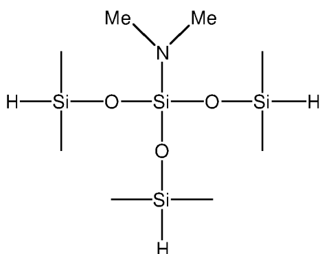
3-dimethylamino-3-(dimethylsiloxy)-1,1,5,5-tetramethyltrisiloxane
