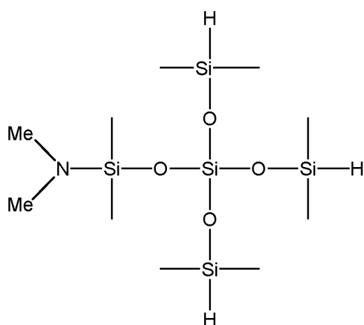
1-dimethylamino-3,3-bis(dimethylsiloxy)-1,1,5,5-tetramethyltrisiloxane
