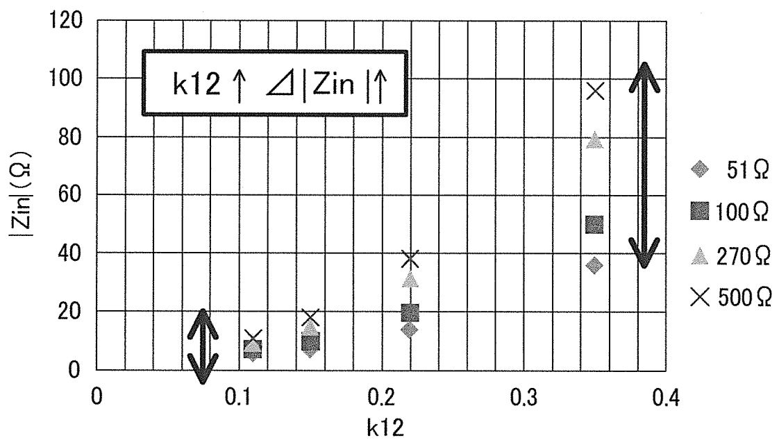
(B) ANTIPHASE RESONANCE MODE
