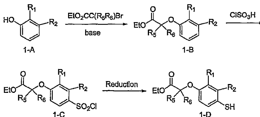
Scheme 1. Synthesis of Intermediate 1-D
