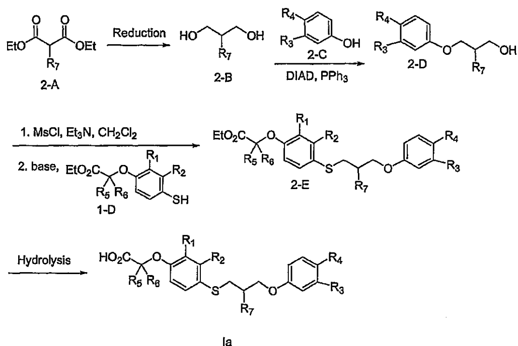
Scheme 2. Synthesis of Compound Ia
