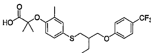
compound 4 #26171158#
