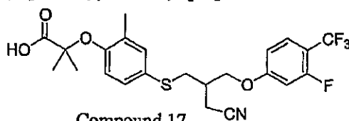
Compound 17
