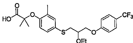
2-{4-[2-Ethoxy-3-(4-trifluoromethyl-phenoxy)-propylsulfanyl]-2-methyl-phenoxy}-2-methyl-propionic acid
