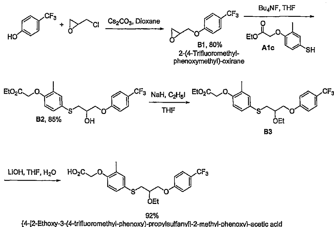
Scheme B
