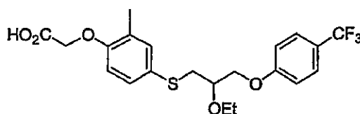
{4-[2-Ethoxy-3-(4-trifluoromethyl-phenoxy)-propylsulfanyl]-2-methyl-phenoxy}-acetic acid
