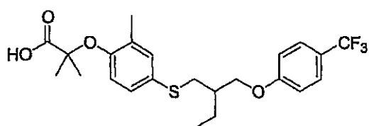
Compound 2
