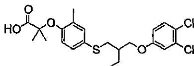
Compound 6
