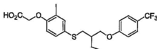
{2-Methyl-4-[2-(4-trifluoromethyl-phenoxy)methyl]-butylsulfanyl}-phenoxy}-acetic acid
