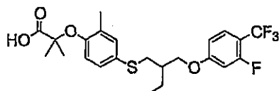
Compound 7
