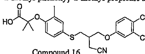
Compound 16
