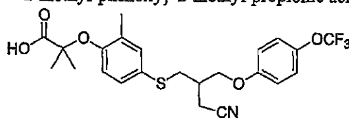
Compound 14
