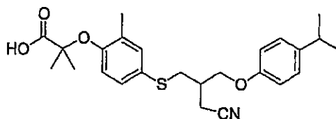
Compound 13
