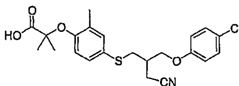
Compound 15
