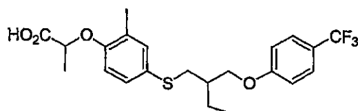
Compound 1
