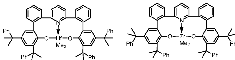
Complex 65
