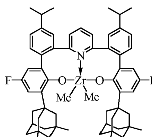
Complex 20
