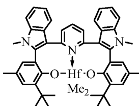
Complex 38
