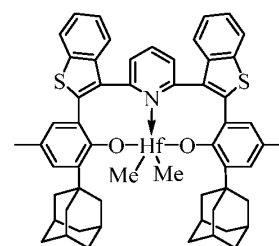
Complex 23
