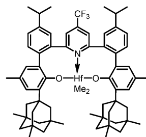
Complex 42
