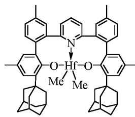
Complex 2
