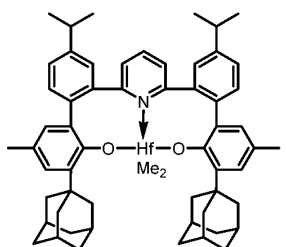
Complex 52
