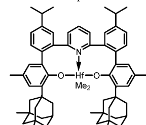
Complex 54
