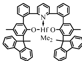
Complex 34
