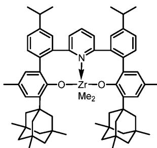
Complex 41
