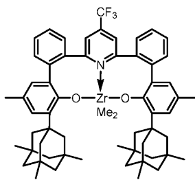
Complex 47
