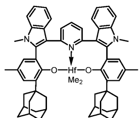
Complex 56
