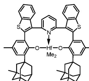
Complex 57
