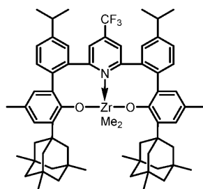
Complex 43
