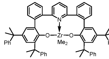
Complex 65
