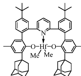
Complex 18
