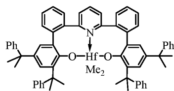
Complex 33
