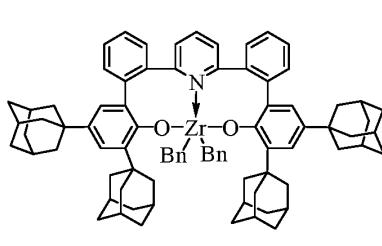
Complex 22
