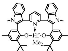
Complex 38
