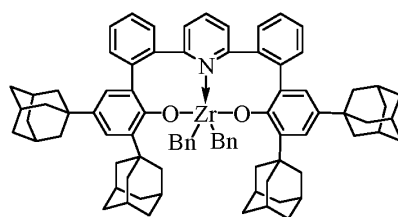
Complex 22
