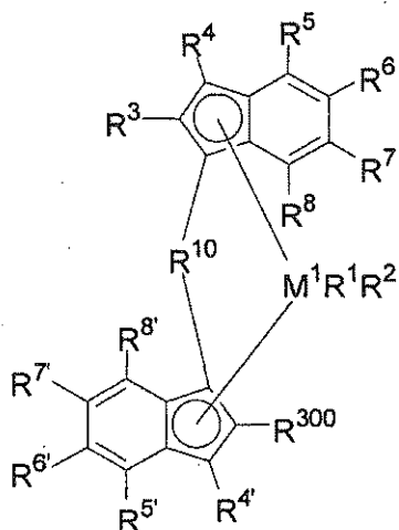
rac/pseudoracemic isomer
