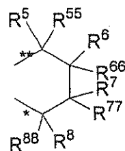
Formula 1 \delta
