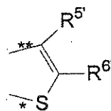
Formula 1 \beta'
