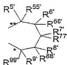
Formula 1v'
