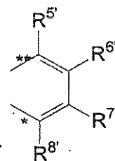
Formula 1 \gamma'
