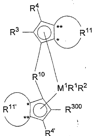
(Formula 1)
