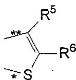
Formula 1 \beta
