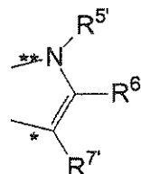
Formula 1 \alpha'
