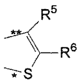
Formula 1 \beta
