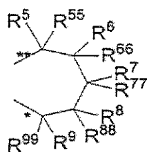
Formula 1v
