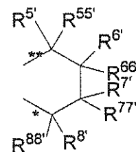
Formula 1 \delta'
