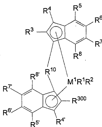
Formula 1a
