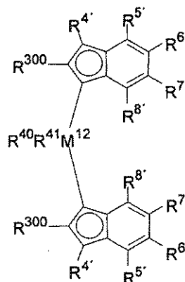
(Formula 4)
