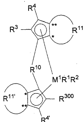
(Formula 1)
