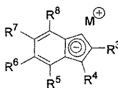
(Formula 5)
