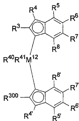
(Formula 6)
