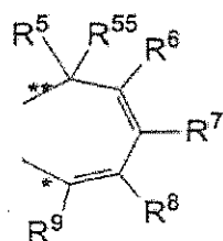
Formula 1φ
