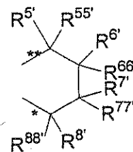
Formula 1 \delta'
