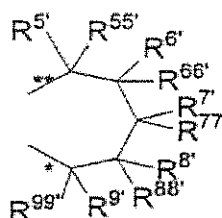
Formula 1ν'
