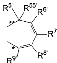
Formula 1φ'
