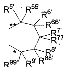
Formula 1v'
