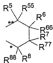
Formula 1 \delta
