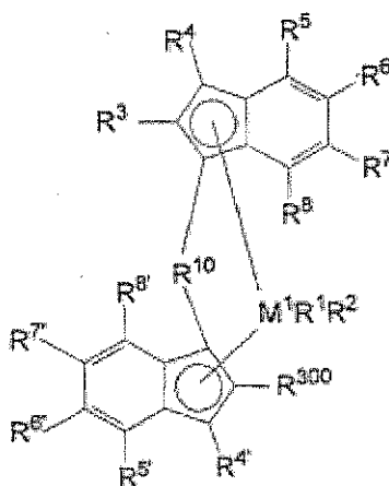
Formula 1a
