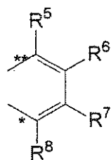
Formula 1 \gamma
