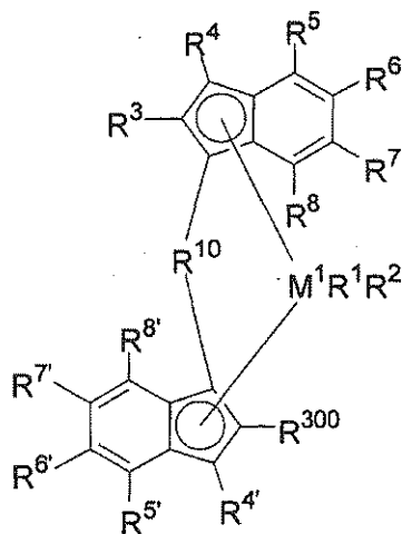
(Formula 1a)
