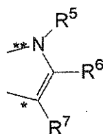
Formula 1 \alpha
