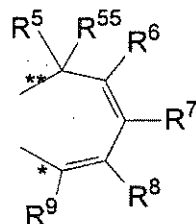
Formula 1φ
