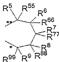
Formula 1ν
