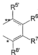
Formula 1 \gamma'
