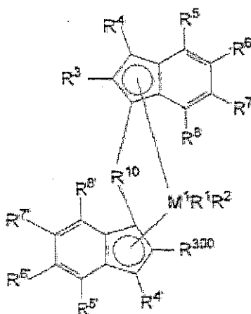
Formula 1a
