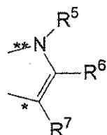
Formula 1 \alpha
