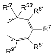
Formula 1φ'
