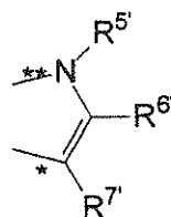
Formula 1 \alpha'
