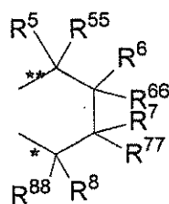
Formula 1δ
