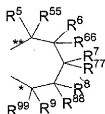
Formula 1v
