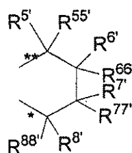
Formula 1δ'
