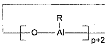
(Formula 8)
