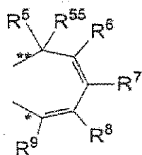
Formula 1φ
