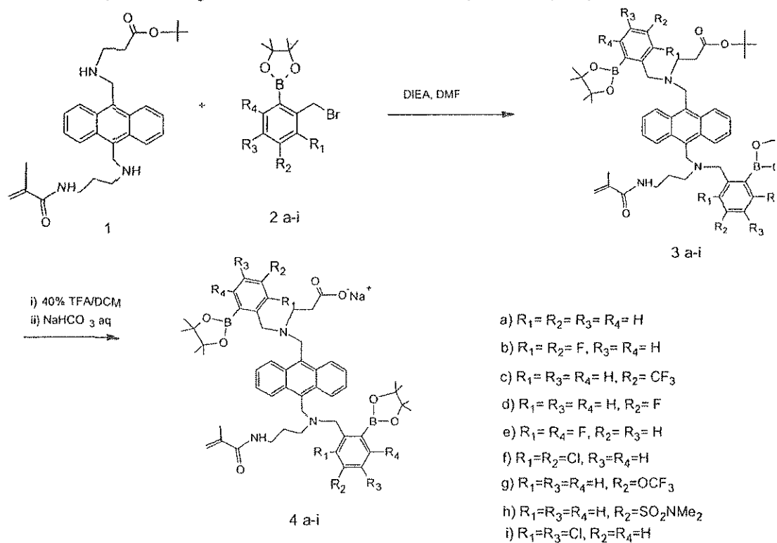
Scheme 2 Synthesis of glucose indicator from commercially available phenylboronic acid
