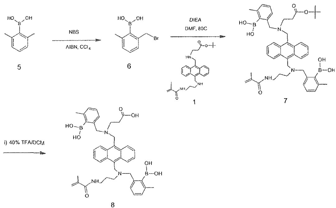
Scheme 2 Synthesis of glucose indicator from commercially available phenylboronic acid
