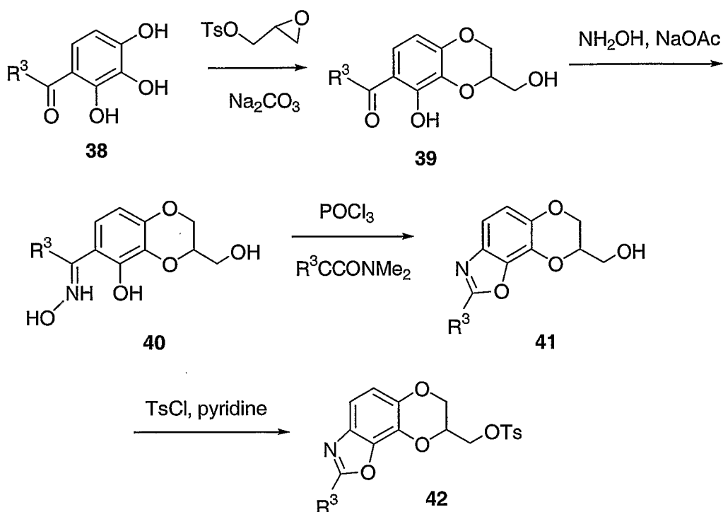
Scheme 13
