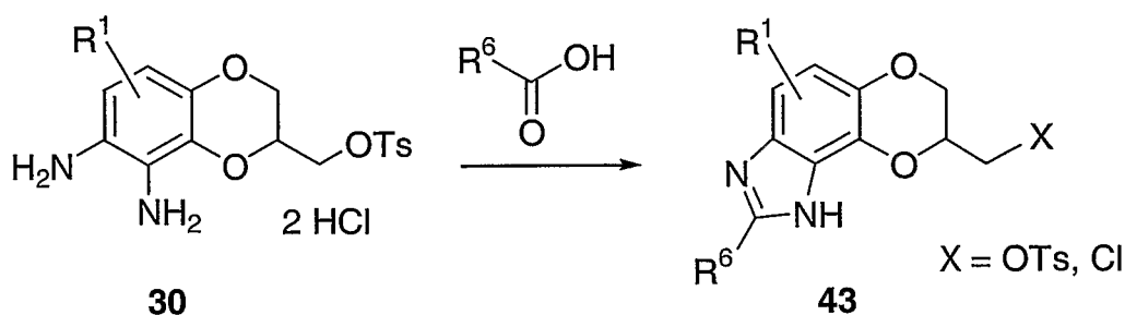
Scheme 14
