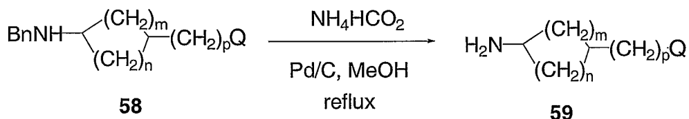
Scheme 19
