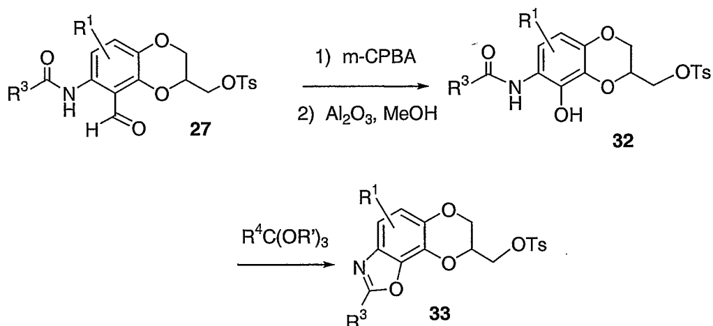
Scheme 11
