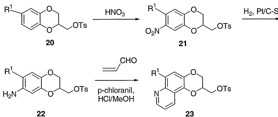
Scheme 7
