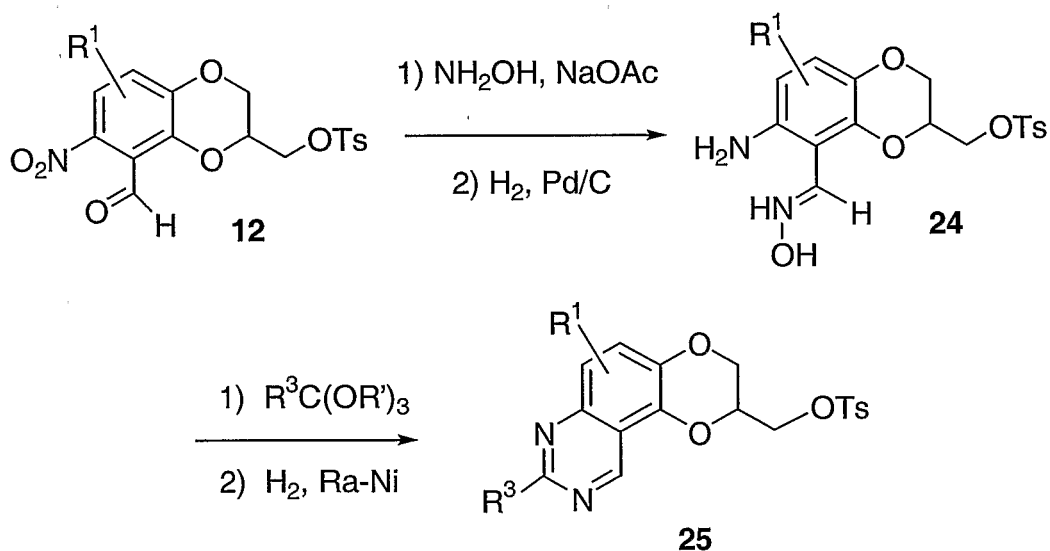
Scheme 8
