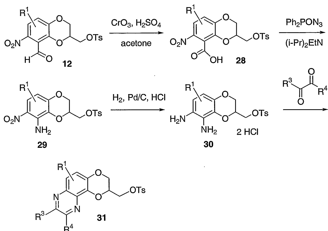
Scheme 10
