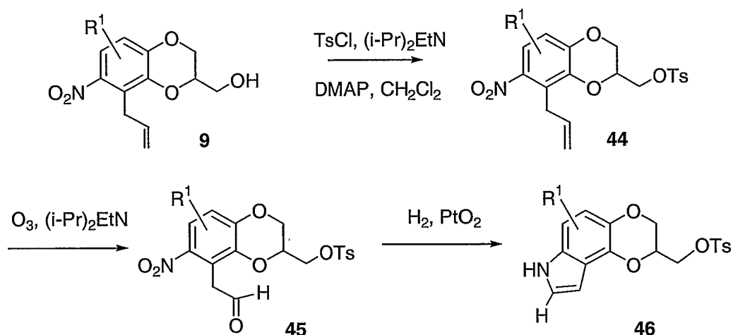
Scheme 15
