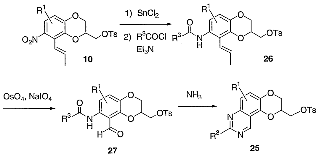
Scheme 9
