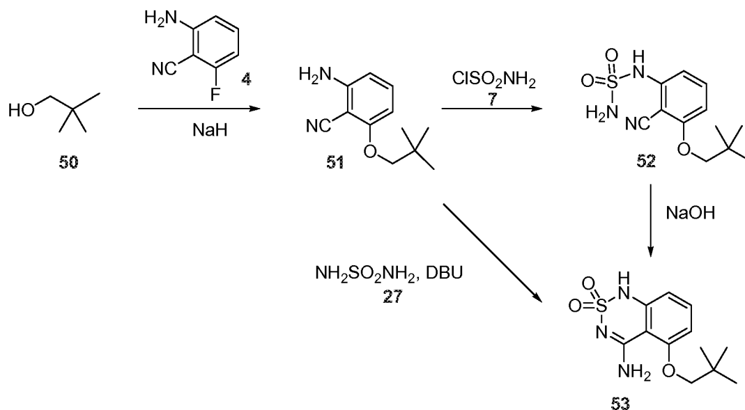
Scheme 17
