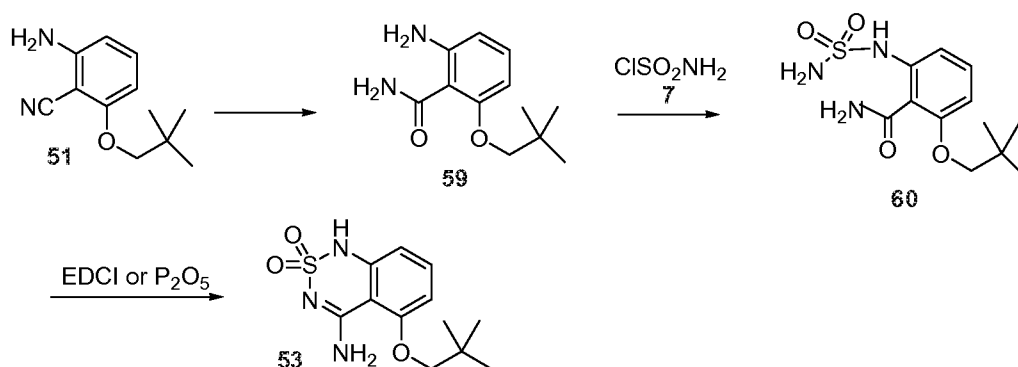
Scheme 21
