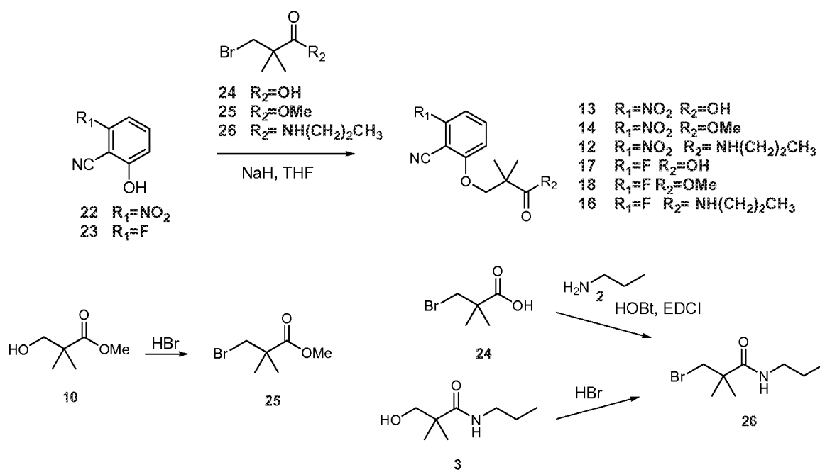
Scheme 10
