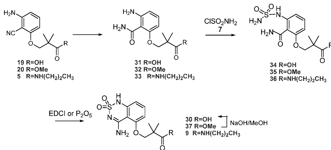
Scheme 14
