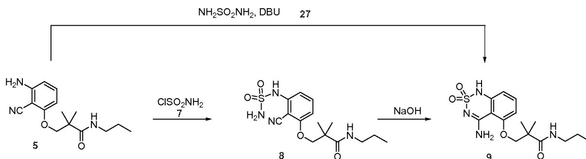
Scheme 12
