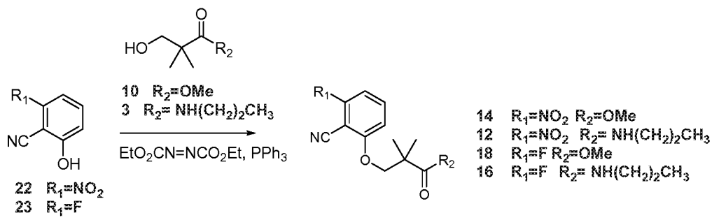
Scheme 11
