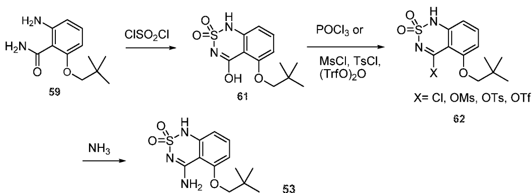
Scheme 22
