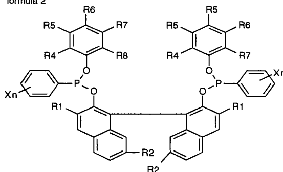
formula 2
