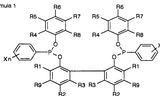
formula 1
