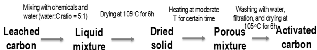
Scheme 1. Schematic diagram for the synthesis of Activated carbon (AC-AP)
