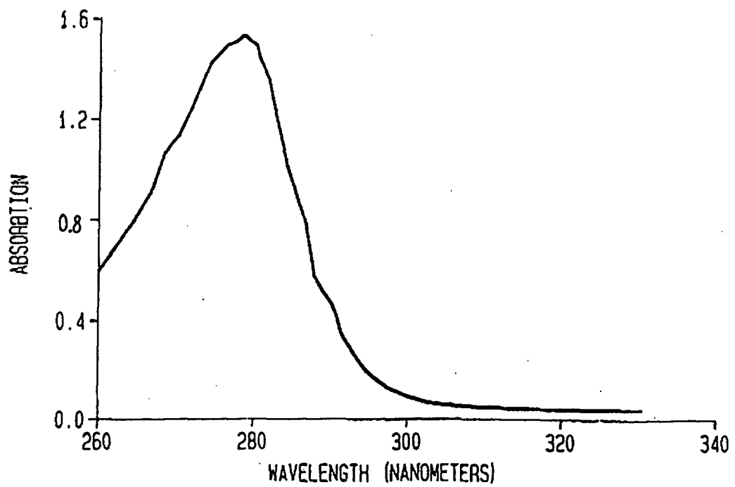
FIG. 2 ABSORPTION OF UV LIGHT BY NONYLPHENOETHOXYLATE SOLUTION @ 500PPM
