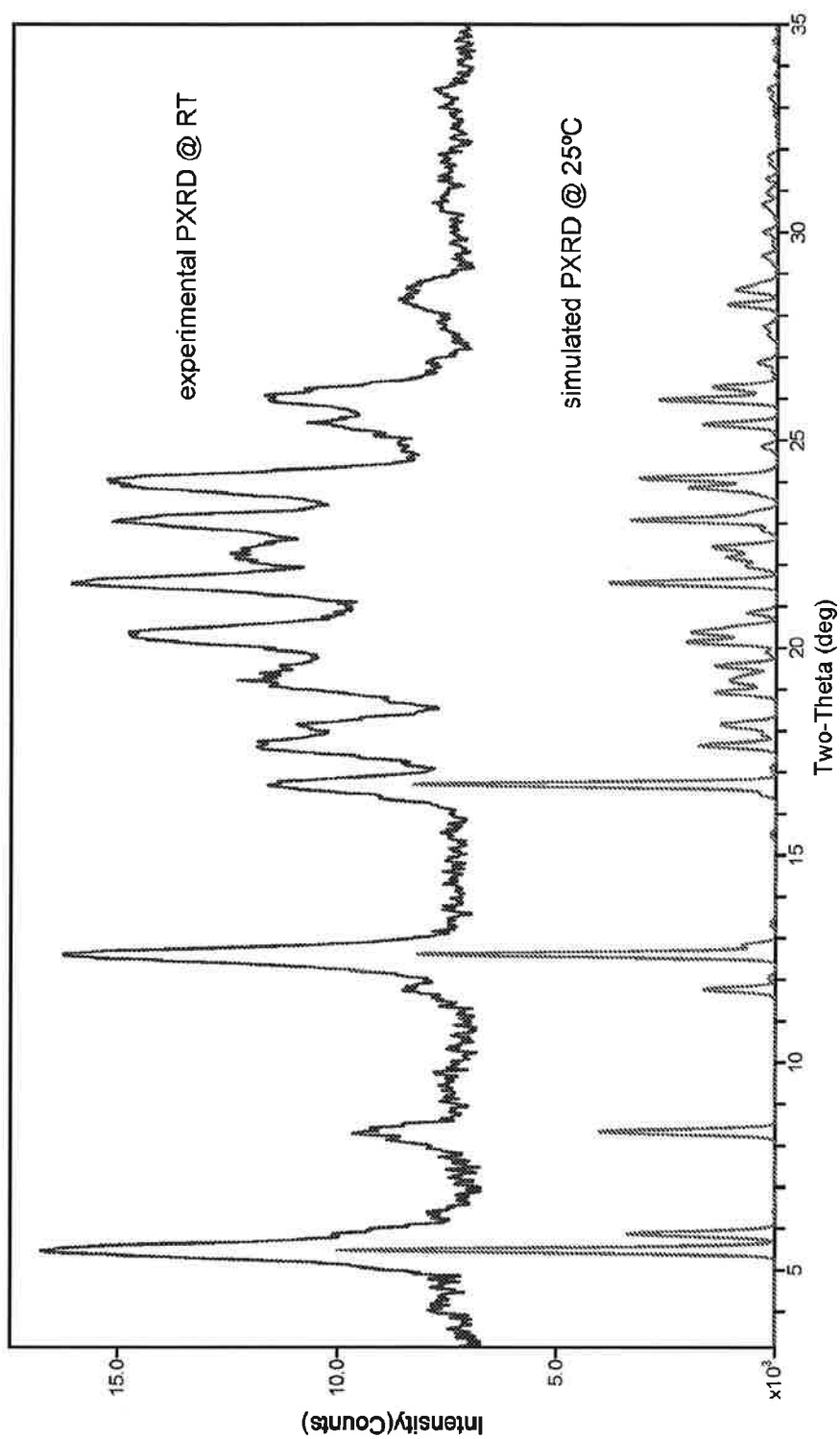
FIG. 13 XRPD of Pattern 3 of Compound 1
