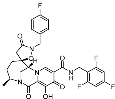
Peak 1
