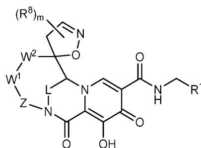
Formula II-A
