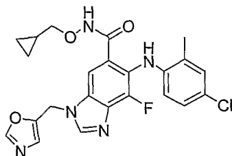
5 6-(4-Chloro-2-methyl-phenylamino)-7-fluoro-3-oxazol-5-ylmethyl-3H-benzimidazole-5-carboxylic acid cyclopropylmethoxy-amide (18ggg)
