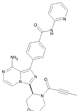
(R)-4-(8-Amino-3-(4-but-2-ynoylmorpholin-3-yl)imidazo[1,5-a]pyrazin-1-yl)-N-(pyridin-2-yl)benzamide
