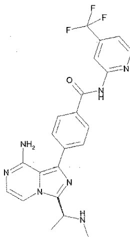
10 (S)-4-(8-Amino-3-(1-(methyamino)ethyl)imidazo[1,5-a]pyrazin-1-yl)-N-(4-(trifluoromethyl)pyridin-2-yl)benzamide
