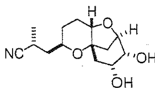
Compound AJ
