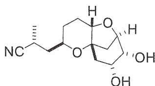
Compound AJ
