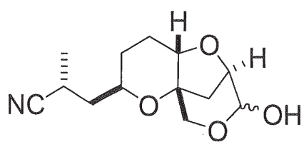
Compound AM.
