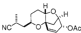
Compound AL
