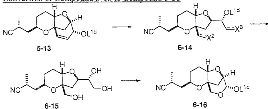
Scheme 6
