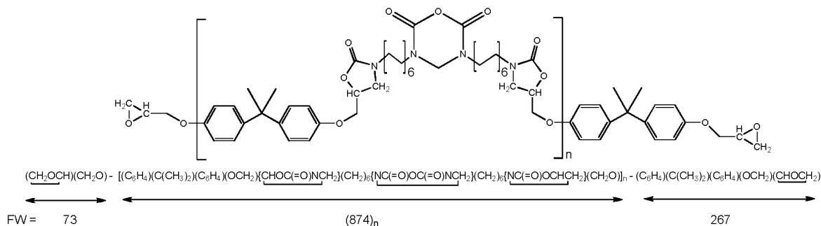
Figure: Representative example of the polyoxazolidinone structure of System 2.
