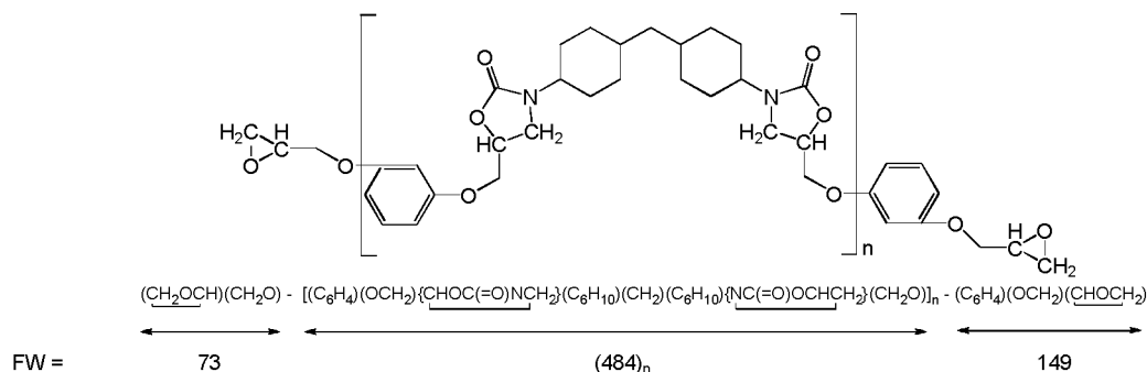
Figure: Representative example of the polyoxazolidinone structure of System 4.
