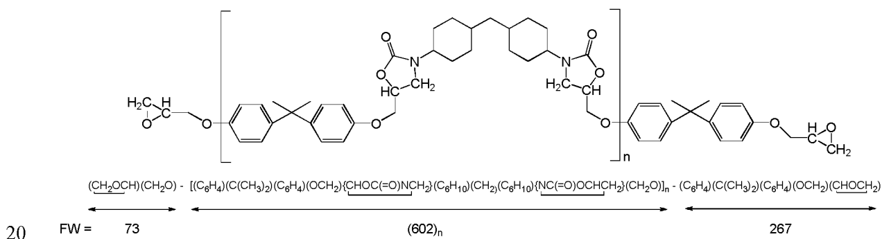
Figure: Representative example of the polyoxazolidinone structure of System 1.
