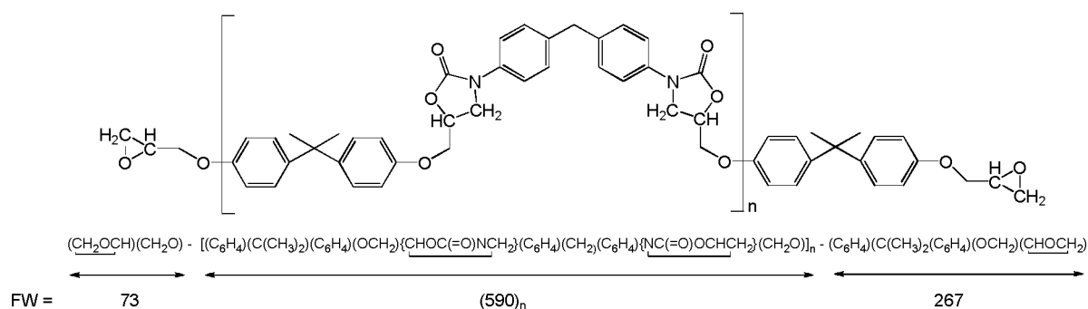
Figure: Representative example of the polyoxazolidinone structure of System 3.
