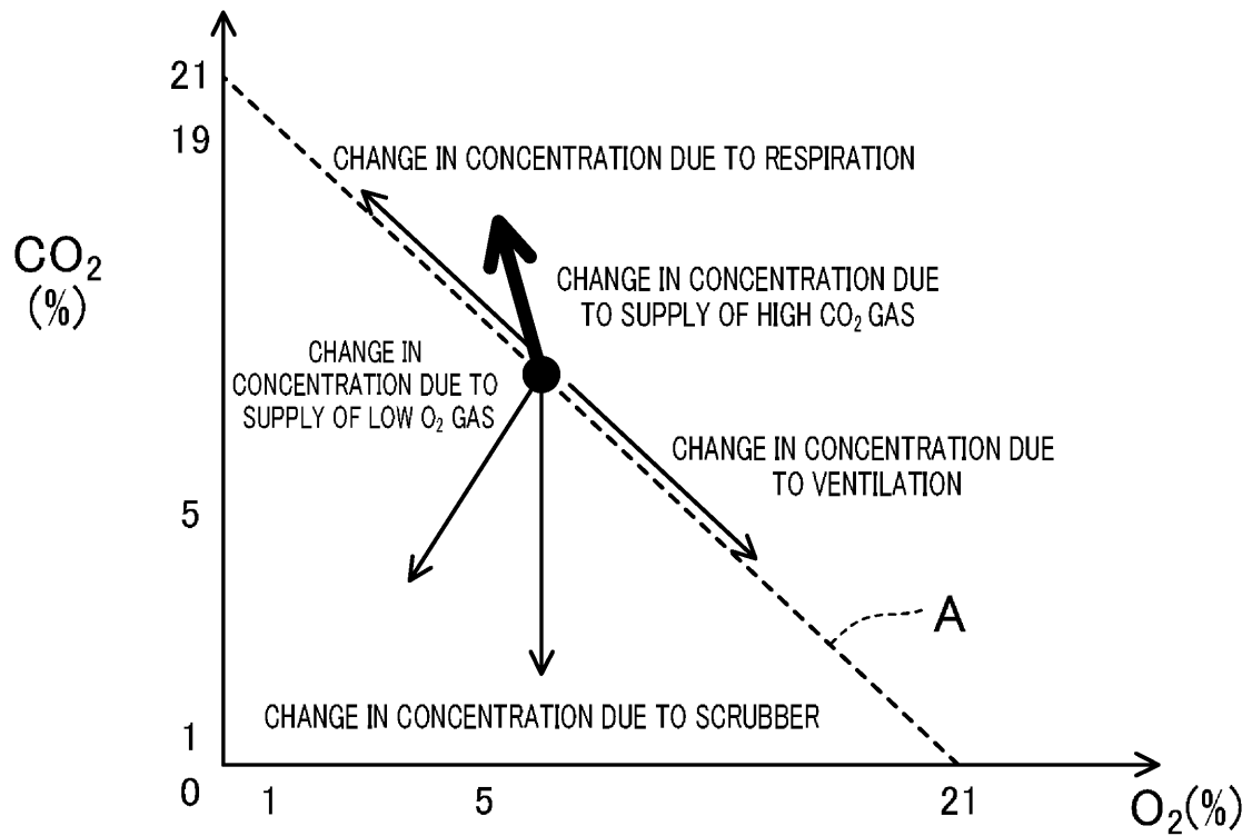
GRAPH 1_CA MACHINE CONTROLLABLE RANGE
