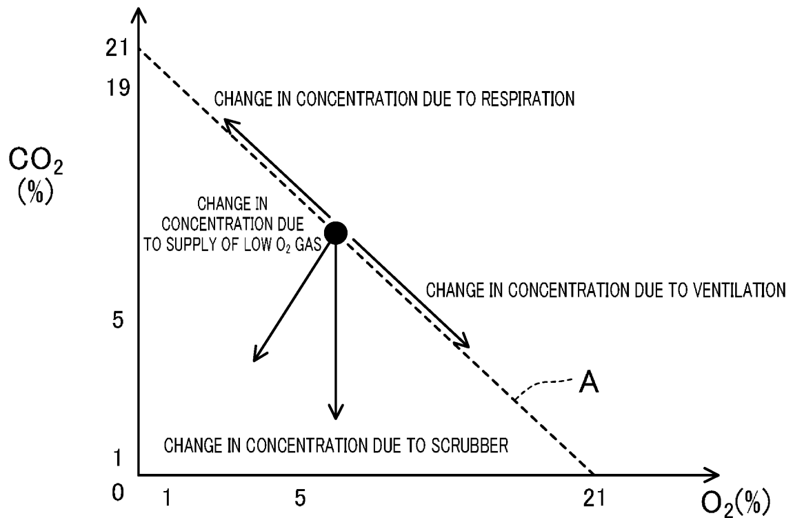
GRAPH 1_CA MACHINE CONTROLLABLE RANGE
