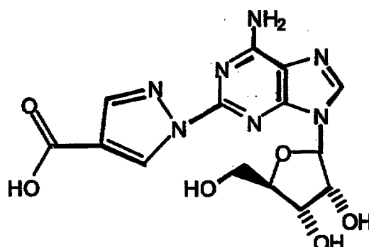
1-{9-[(4S,2R,3R,5R)-3,4-dihydroxy-5-(hydroxymethyl)oxolan-2-yl]-6-aminopurin-2-yl}pyrazole-4-carboxylic acid (17)
