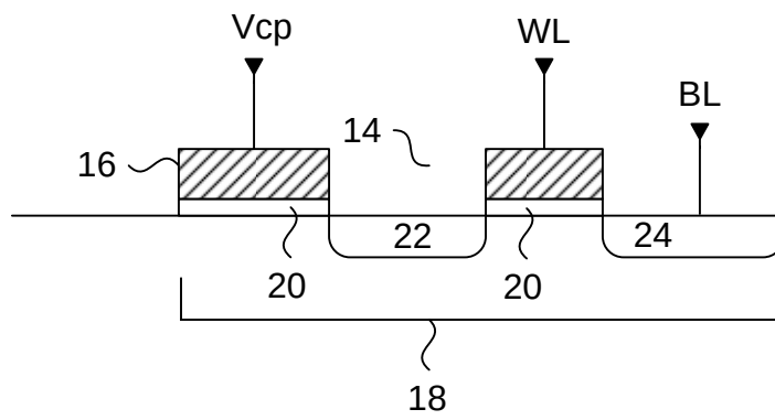
FIG. 3 (Prior Art)
