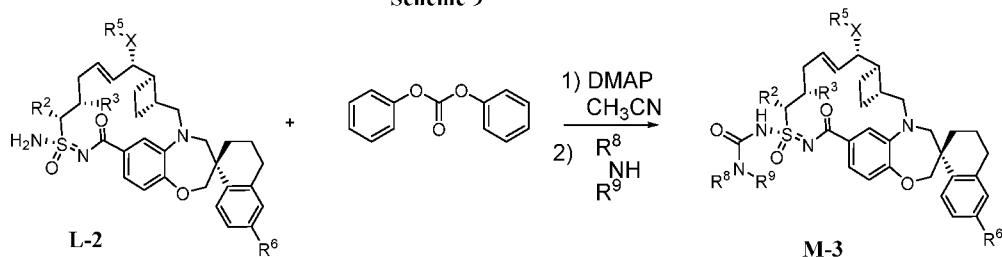
Scheme 9
