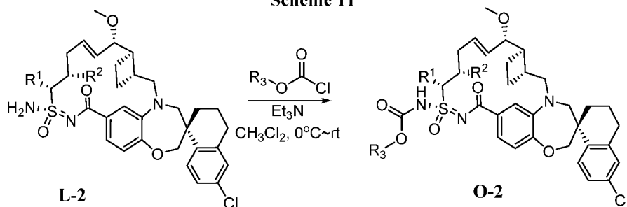
Scheme 11
