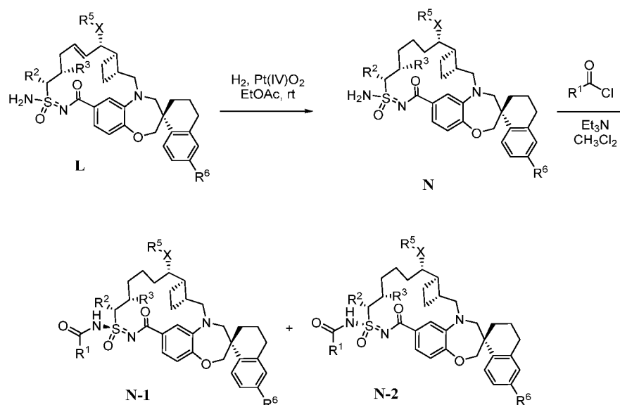
Scheme 6
