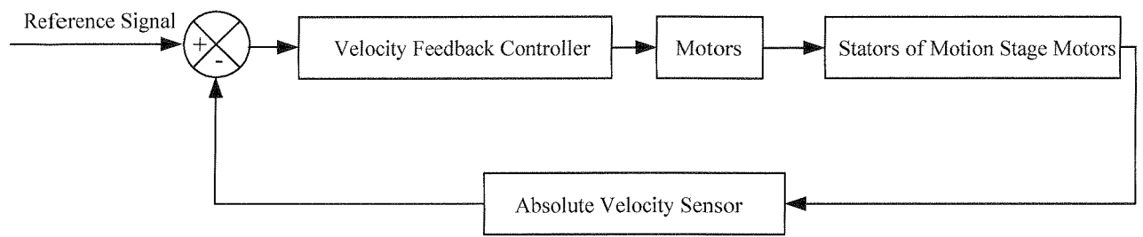
Absolute Velocity Feedback Loop
