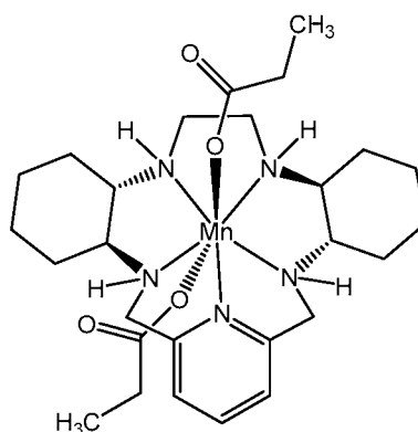
[Bis-Propionato(GC4419)] \text{C}_{27}\text{H}_{45}\text{MnN}_5\text{O}_4 MW 558.63
