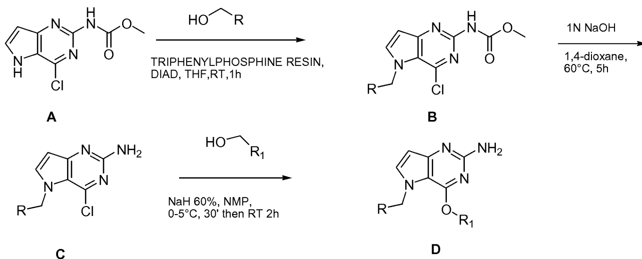
Scheme 1. Overall reaction scheme
