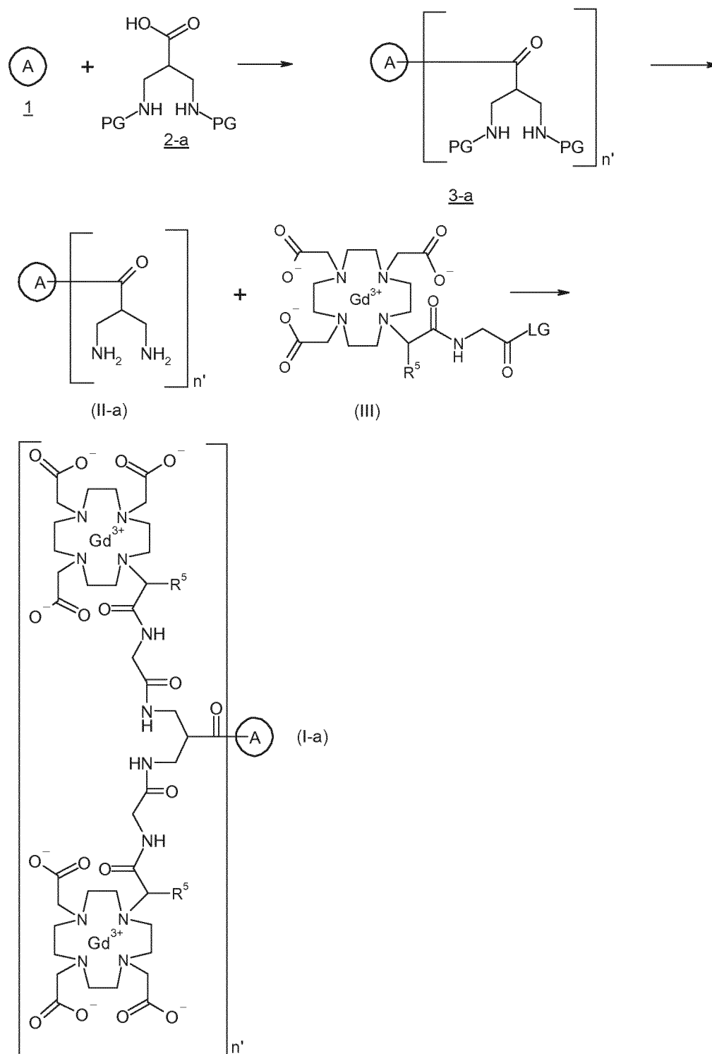
5 Scheme 1: Route for the preparation of compounds of general formula (I-a), wherein
