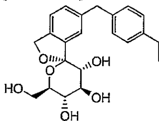
[Formula 20]
