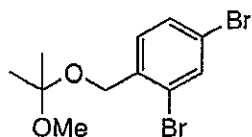
[0113] [Formula 17]
