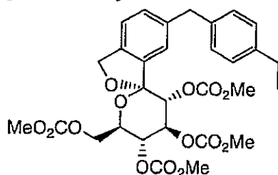
[Formula 21]
