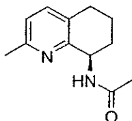
(R) -N-(2-Methyl-5,6,7,8-tetrahydroquinolin-8-yl)-acetamide
