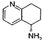
(S) -5-Amino-5,6,7,8-tetrahydroquinoline
