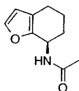
5 (R)-N-(4,5,6,7-tetrahydrobenzofuran-7-yl)acetamide
