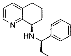
(1-(R)-1-Phenylpropyl)-(8-(R)-5,6,7,8-tetrahydroquinolin-8-yl)-amine
