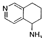
(R,S)-5-Amino-5,6,7,8-tetrahydroisoquinoline
