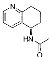
(S)-6-Amino-5,6,7,8-tetrahydroquinoline
