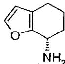
5 (R)-N-(4,5,6,7-tetrahydrobenzofuran-7-yl)acetamide
