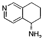
(S)-5-Amino-5,6,7,8-tetrahydroisoquinoline
