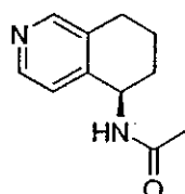
(R)-N-(5,6,7,8-tetrahydro-isoquinolin-5-yl)-acetamide
