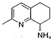
(S) -8-Amino-2-methyl-5,6,7,8-tetrahydroquinoline
