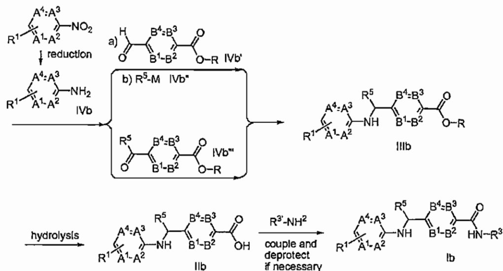
Reaction Scheme IV
