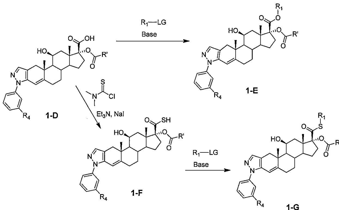
[0141] Scheme 2:
