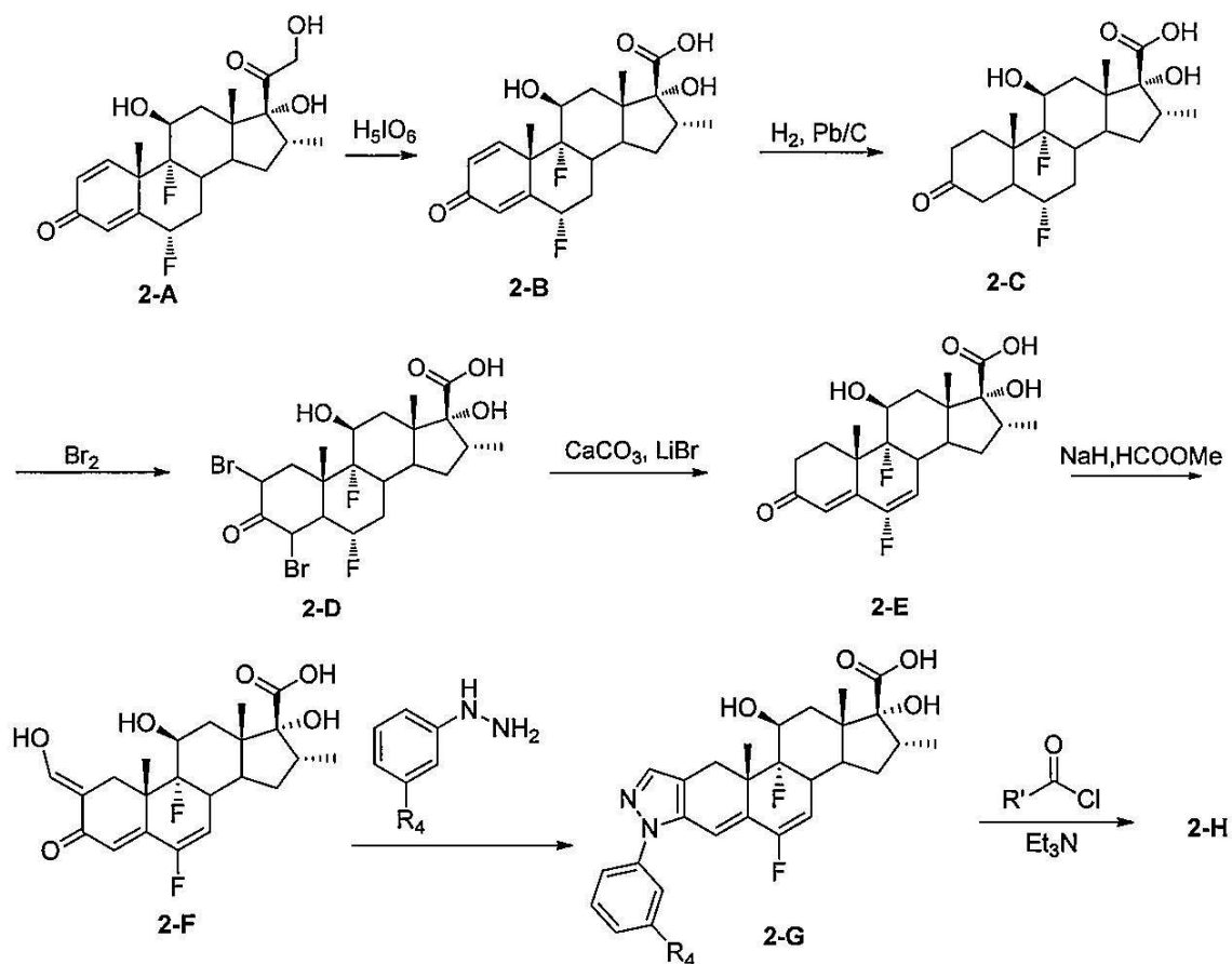
[0144] Scheme 3:
