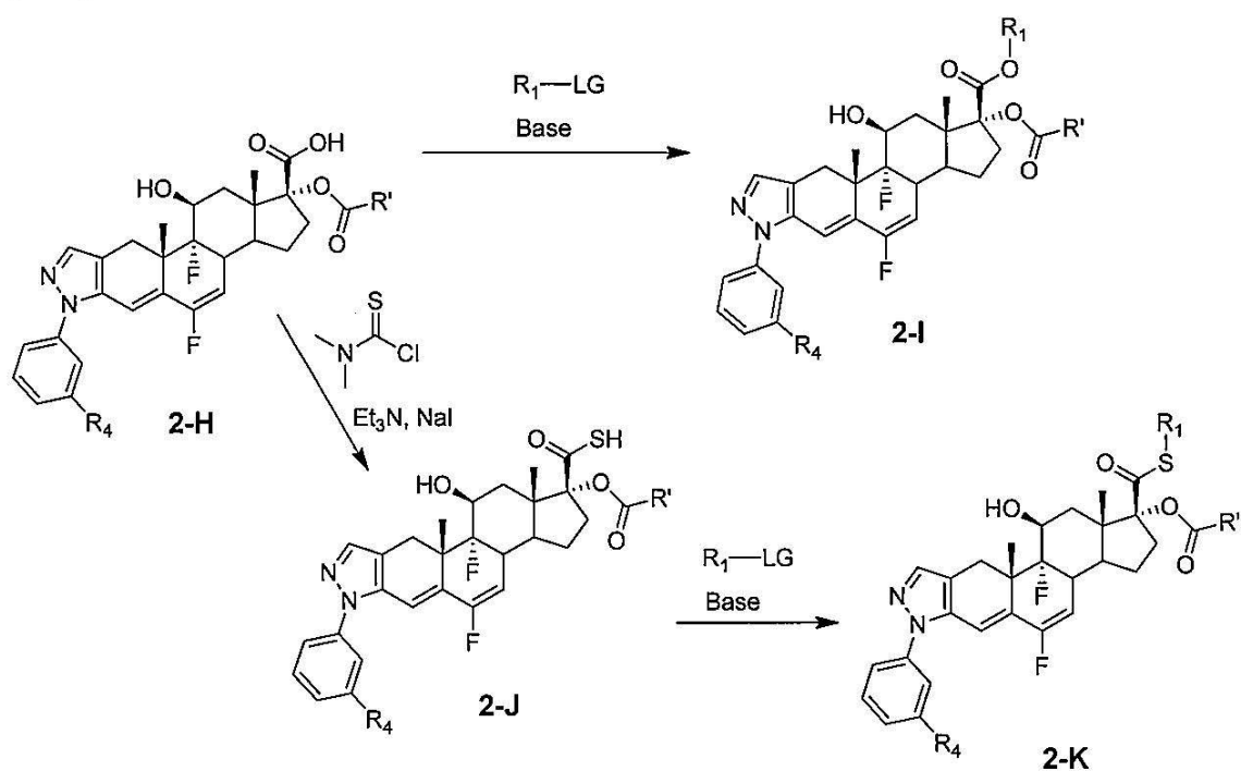
[0145] Scheme 4:
