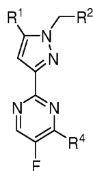
Formula I
