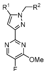
Formula II
