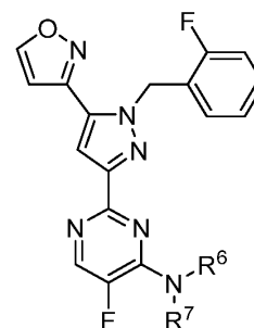
Formula VII
