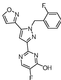
( 9' ) ; and
