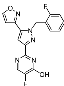
Compound 9'
