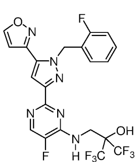
Formula IA
