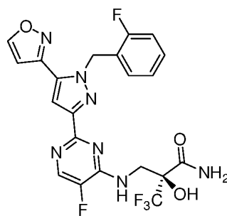
Formula IC,
