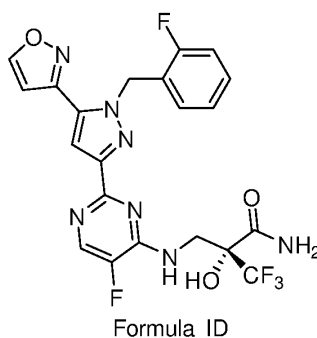
Formula ID,
