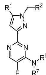
Formula IV
