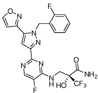
Formula ID
