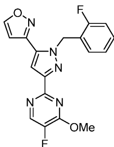
Formula V
