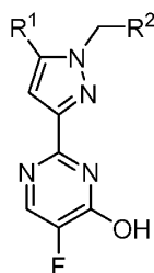
Compound 9
