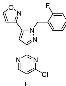
Formula VI
