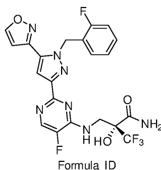
Formula ID,
