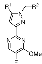
Formula II
