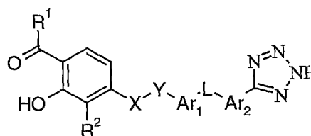
tautomer II
