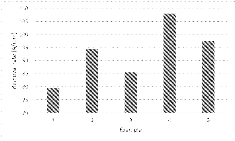
FIG. 3. SiN Film Removal Rates
