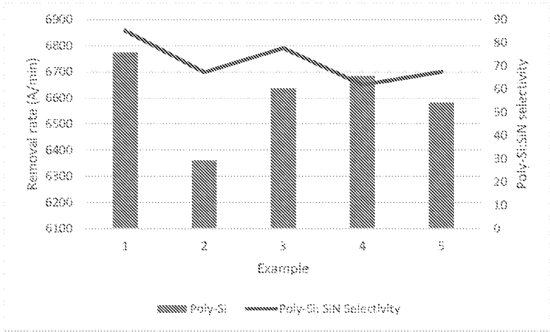
FIG. 2. Film Removal Rates and Poly-Si: SiN Selectivity
