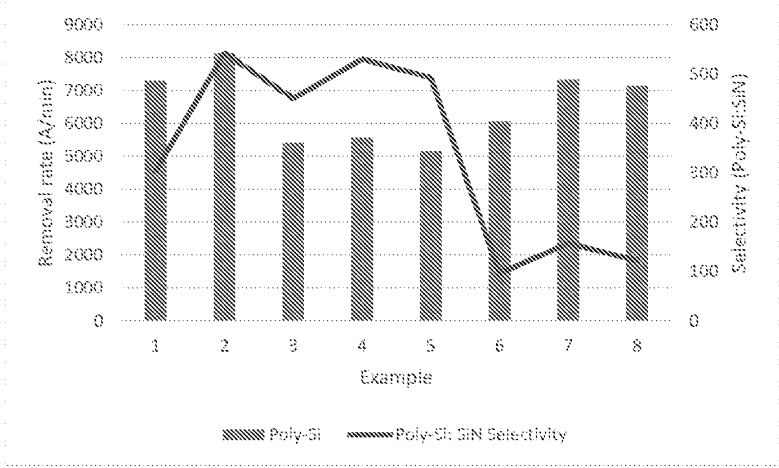
FIG. 1. Film Removal Rates and Poly-Si: SiN Selectivity
