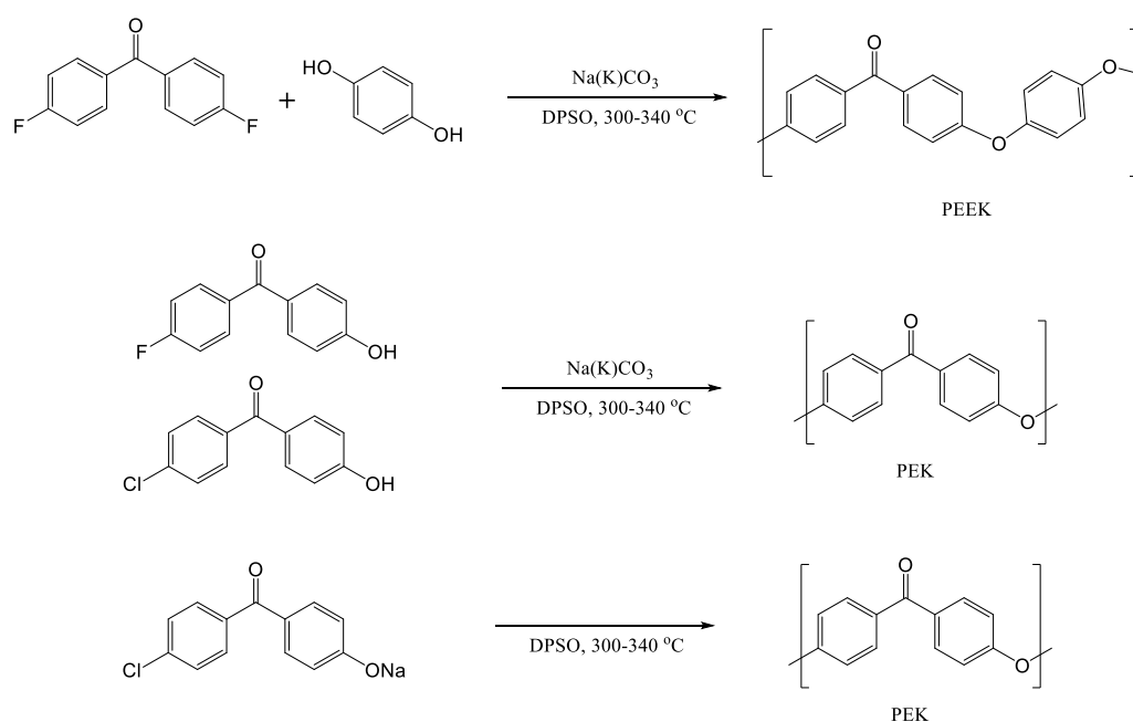
Scheme 1. Typical PAEKs (PEEK and PEK) synthesis route.
