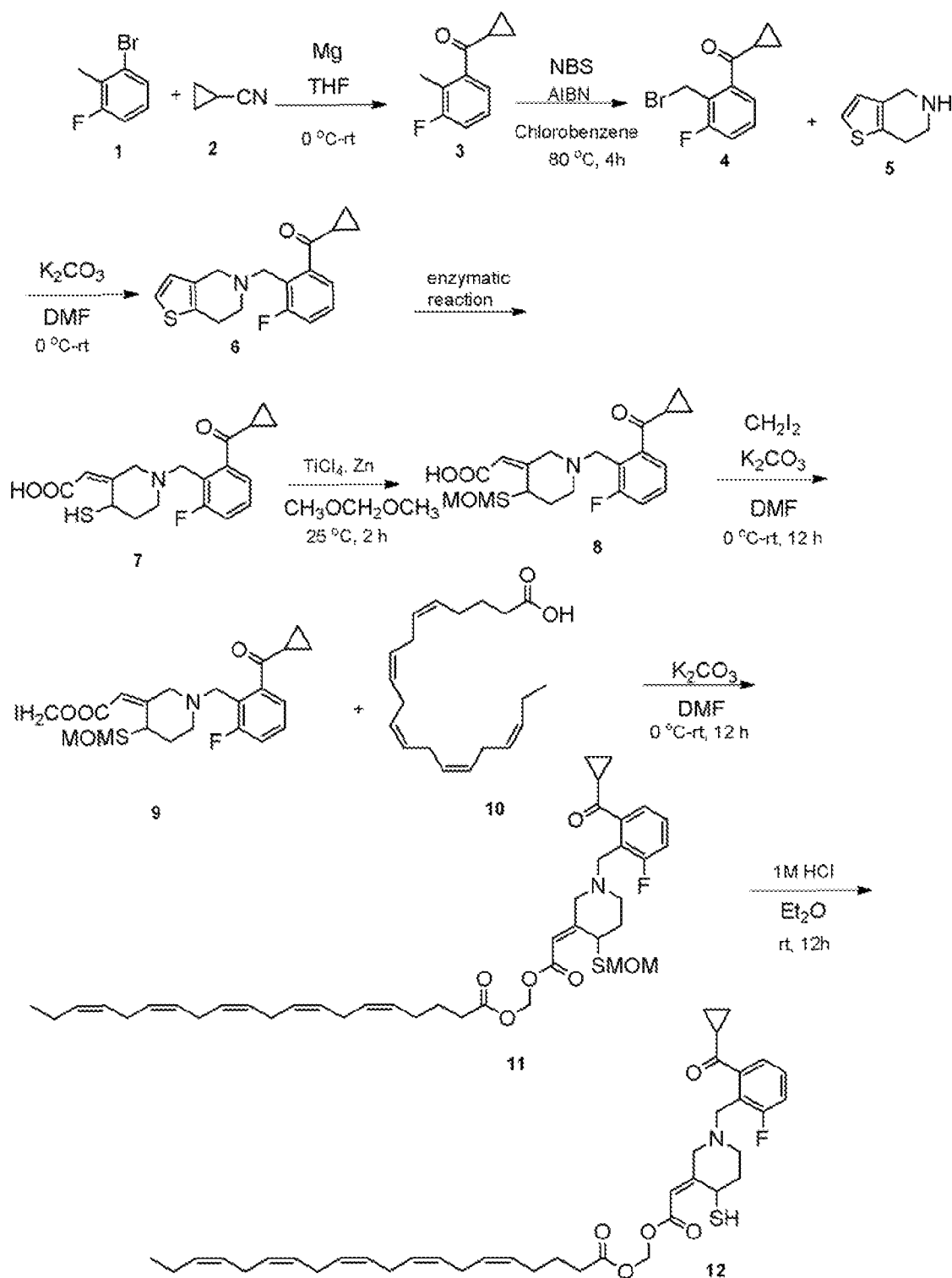
Scheme – 2:
