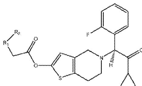
Formula II
