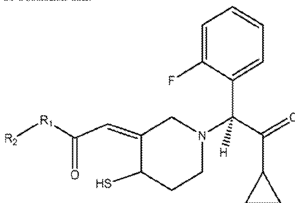
Formula IIa
