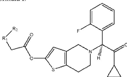
Formula II
