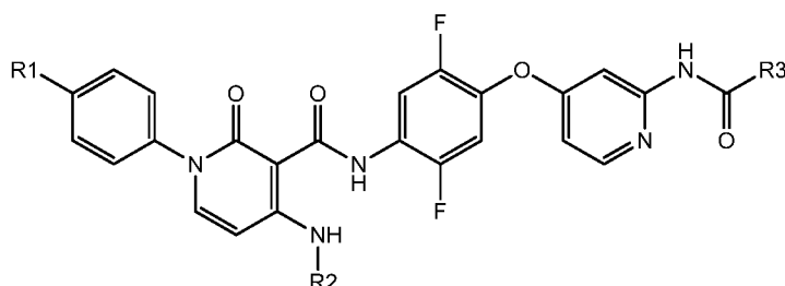
Formula If
