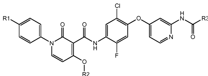
Formula Ig.5
