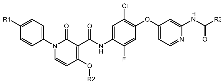
Formula Ig.6
