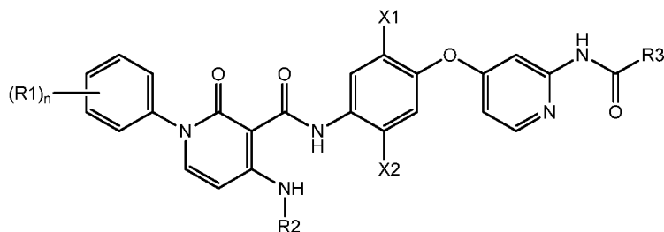
Formula Id.2
