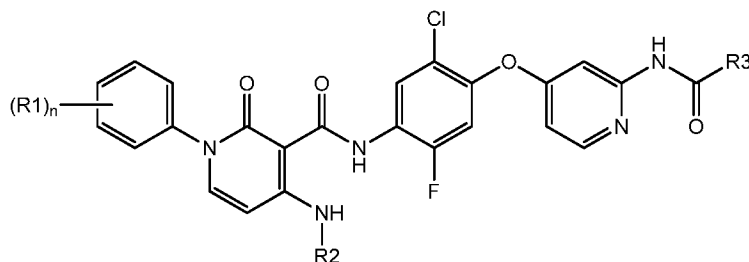
Formula 1h
