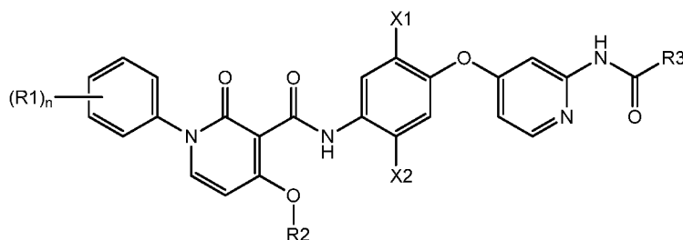
Formula Ia
