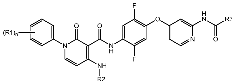
Formula Ie.4
