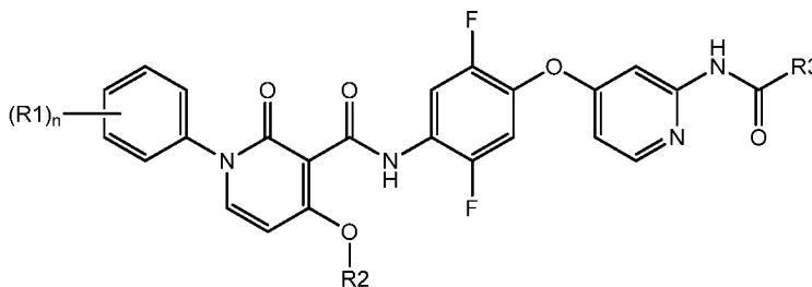
Formula Ib.3
