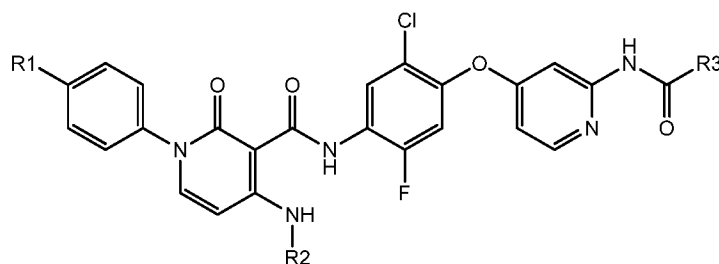
Formula Ih.5
