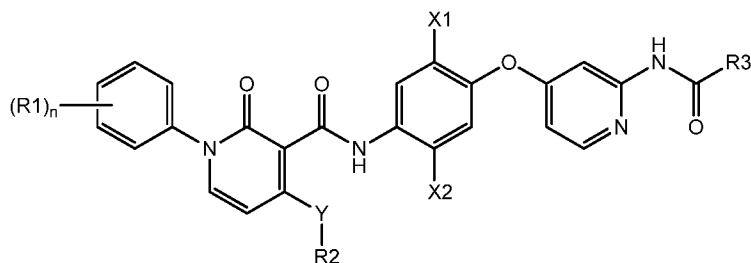
Formula I.2
