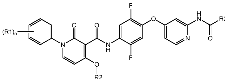
Formula Ib.2
