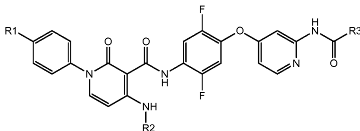
Formula If.1
