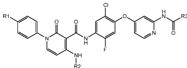
Formula Ih.6
