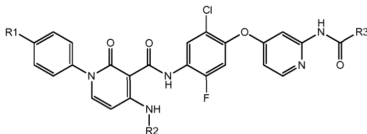
Formula Ih.3
