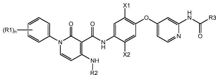
Formula Id.3
