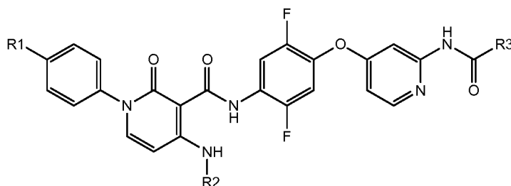
Formula If
