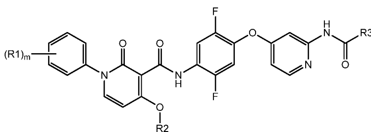
Formula Ib
