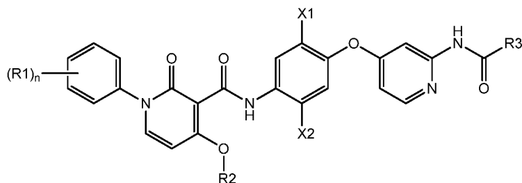
Formula Ia.4
