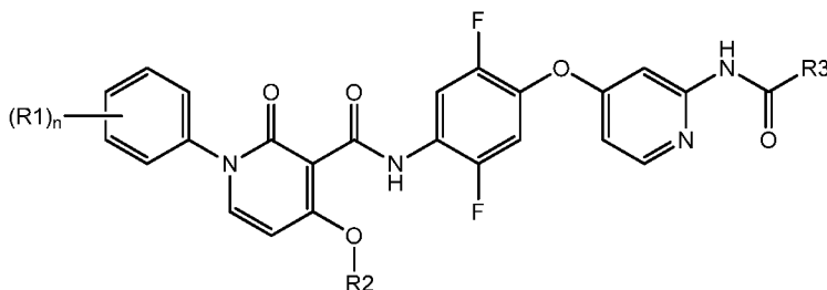
Formula Ib.4
