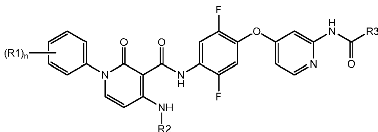
Formula Ie
