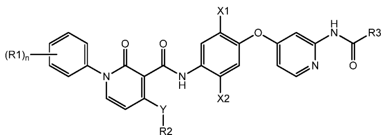
Formula I.4
