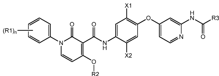
Formula Ia.2
