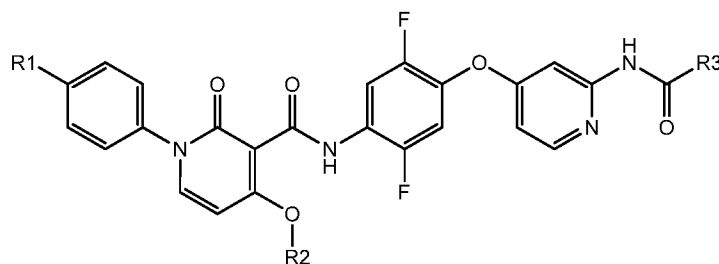
Formula Ic.4
