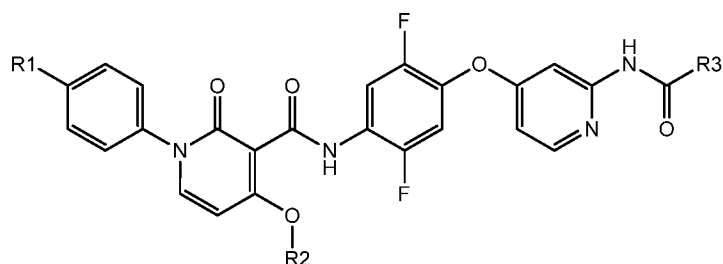
Formula Ic.1
