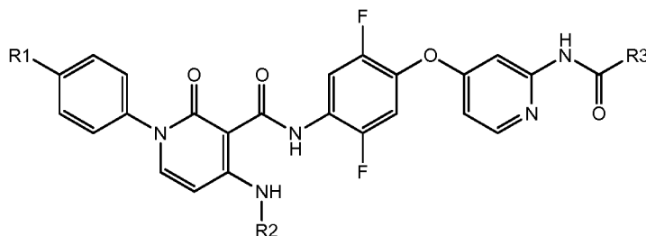
Formula If.5
