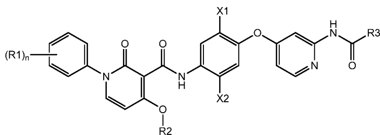
Formula Ia.3
