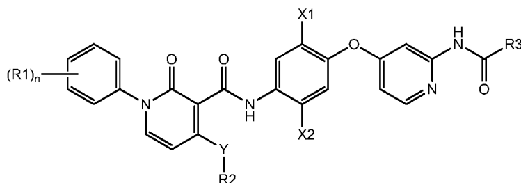
Formula I.1
