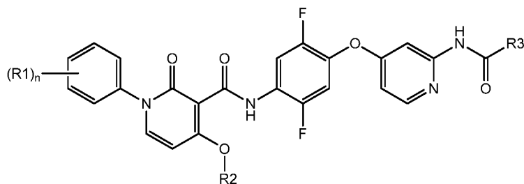
Formula Ib
