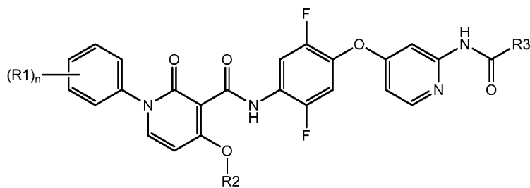
Formula Ib.1
