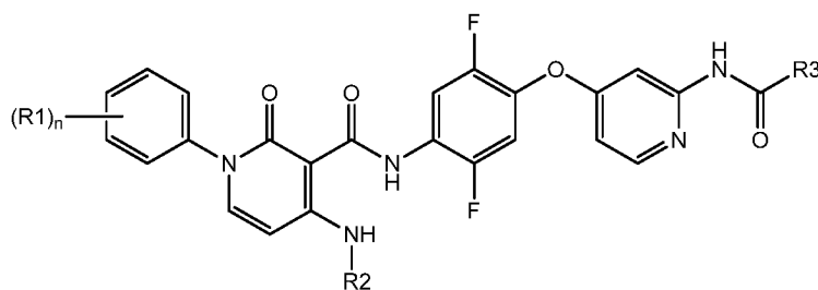
Formula Ie
