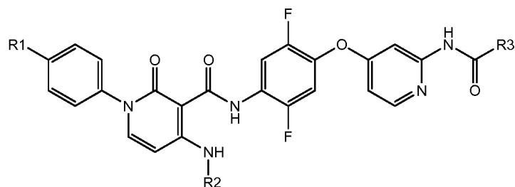
Formula If.4
