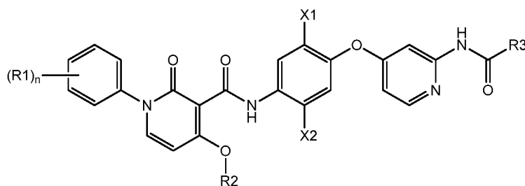
Formula Ia.1
