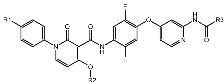
Formula Ic.2
