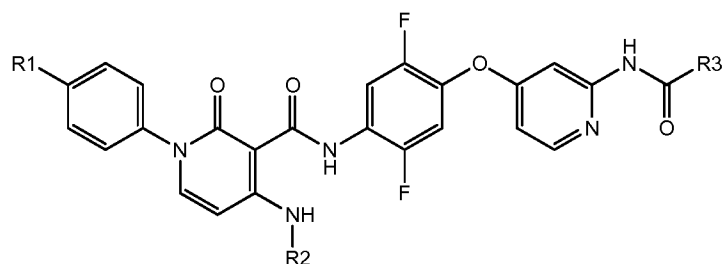
Formula If.3
