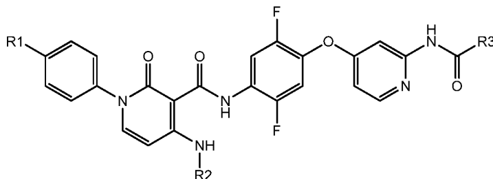
Formula If.6
