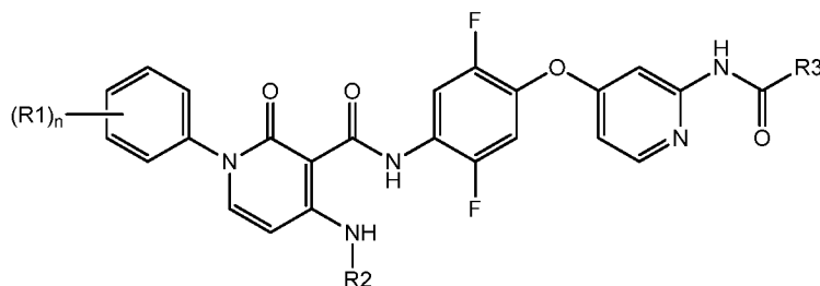
Formula Ie.3
