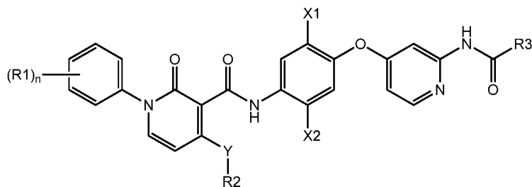
Formula I.3
