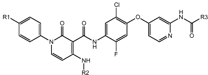
Formula Ih.2
