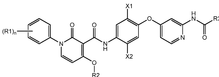
Formula Ia
