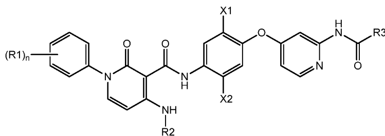
Formula Id.1
