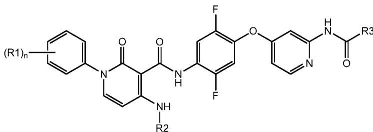
Formula Ie.1
