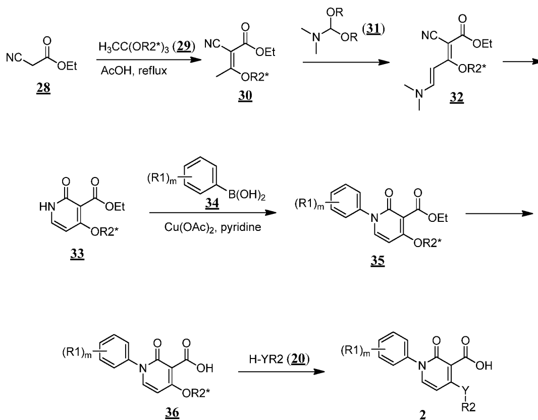
Scheme 6
