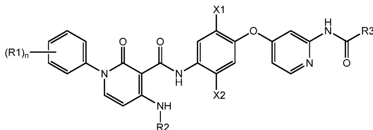
Formula Id
