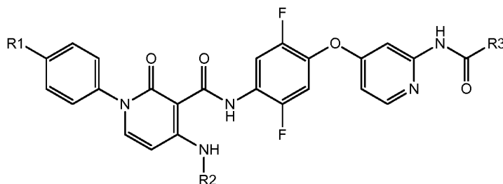
Formula If.2
