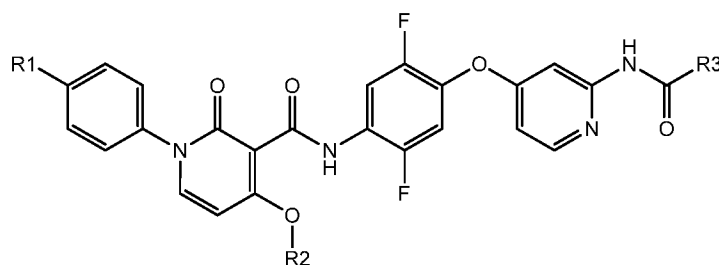
Formula Ic.3
