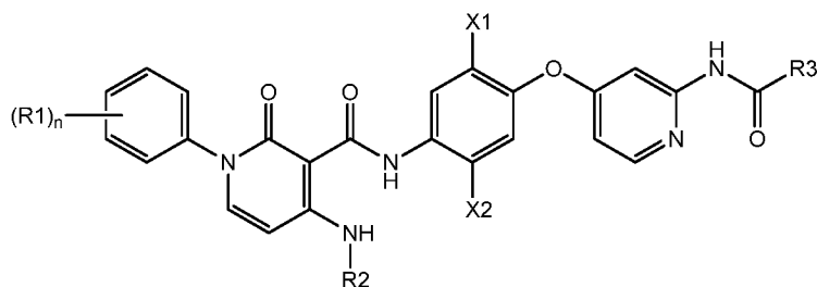
Formula Id.4
