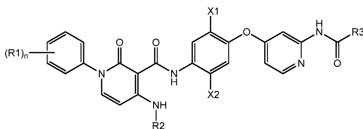
Formula Id
