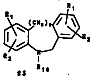
93 ( R_{16}=H ) 5,6,11,12-tetrahydrodibenz[b,f]azocine
