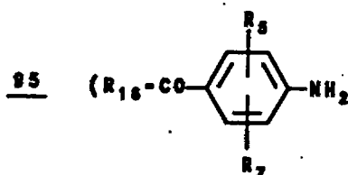
95 ( R_{16}=CO-C_6H_4NH_2 ) 5,6,11,12-tetrahydro-5-(4-aminobenzoyl)dibenz[b,f]azocine
