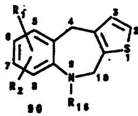
90 ( R_{16}=H ) 4,10-dihydro-9H-thieno[2,3-c][1]benzoxepine
