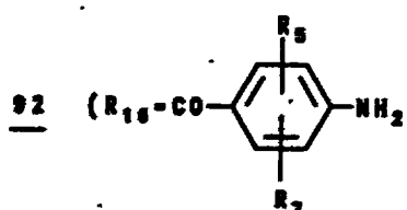
92 ( R_{16}=CO-C_6H_4NH_2 ) 4,10-dihydro-9-(4-aminobenzoyl)-9H-thieno[2,3-c][1]benzoxepine
