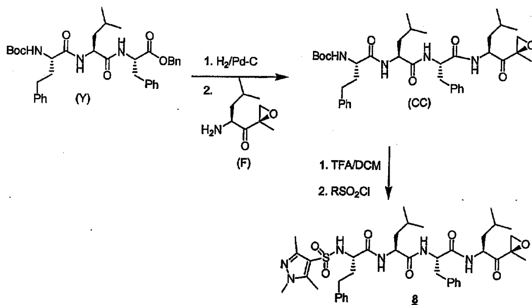
Scheme 8: Synthesis of Example 8
