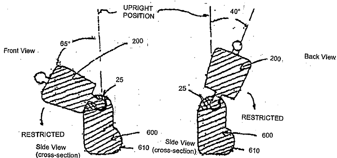
Figure 10A UPPER &amp; LOWER TORSO JOINT
