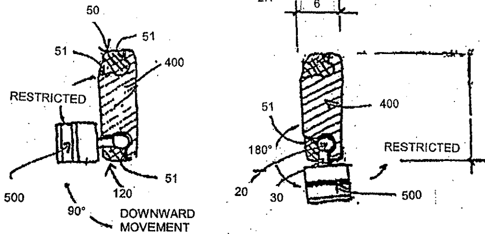
LOWER ARM TO HAND JOINT
