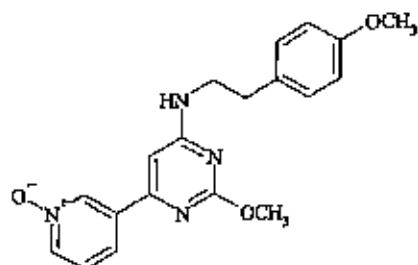
[2-methoxy-6-(1-oxy-pyridin-3-yl)-pyrimidin-4-yl]-[2-(4-methoxy-phenyl)-ethyl]-amine.
