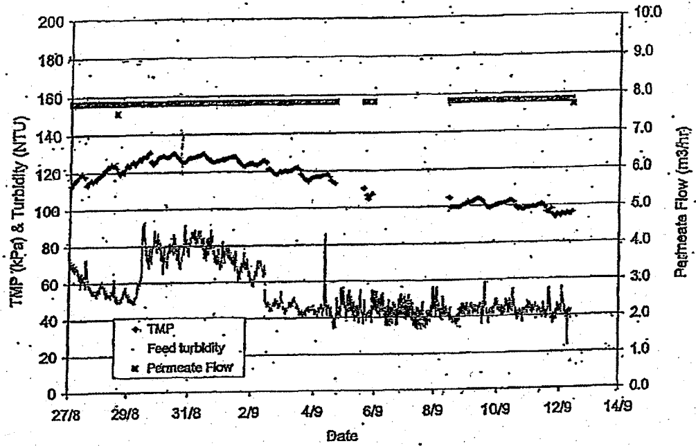
Figure 2 Membrane Filtration Performance with Air Pushed Backwash
